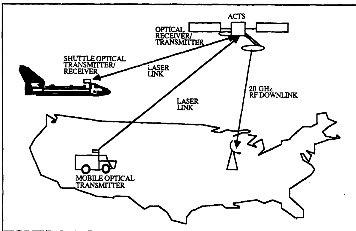
Figure 3.8 The ACTS Optical Intersatellite Links [ Ref. 8: p. 13 ]
