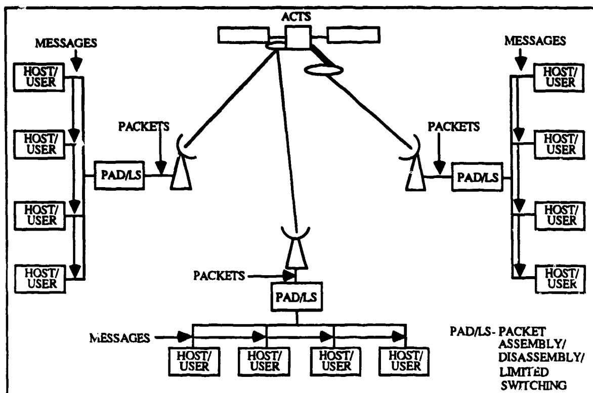
Figure 5.3 ACTS System Used with Clustered Hosts
