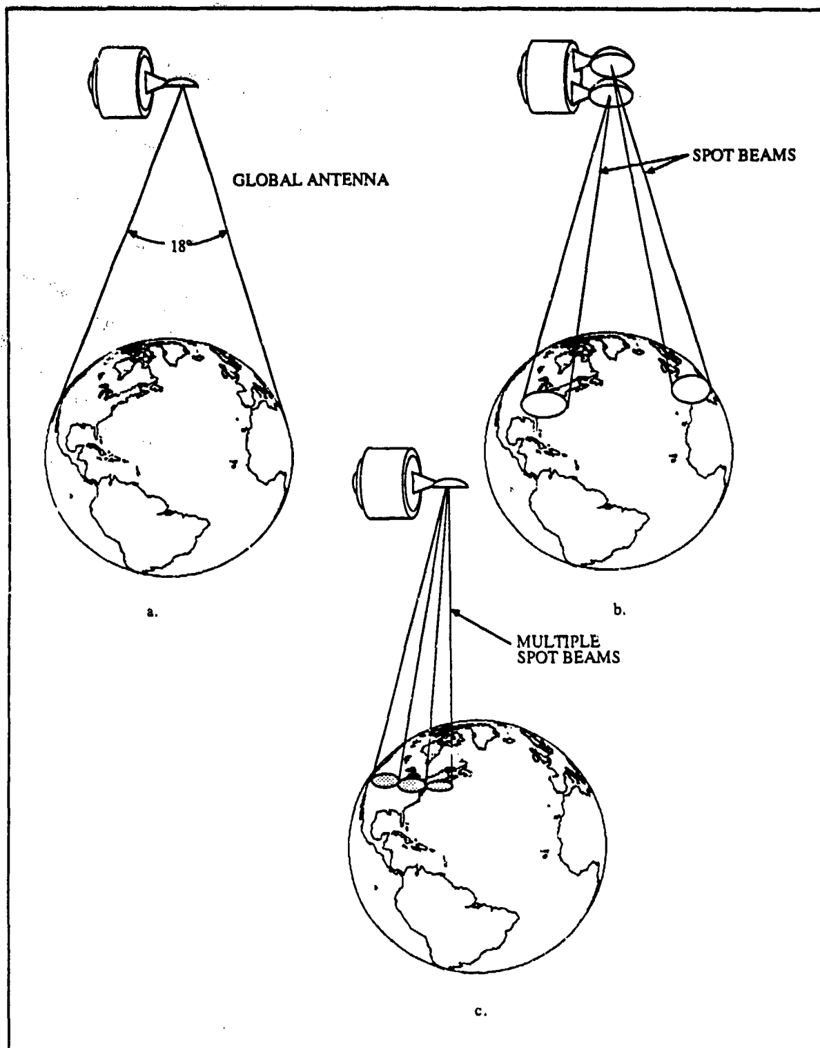
Figure 2.9 Antenna Beams [ Ref. 3: p. 127 ]
