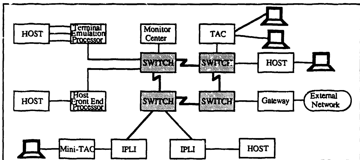
Figure 4.3 DDN Components [ Ref. 33: p. 7 ]
