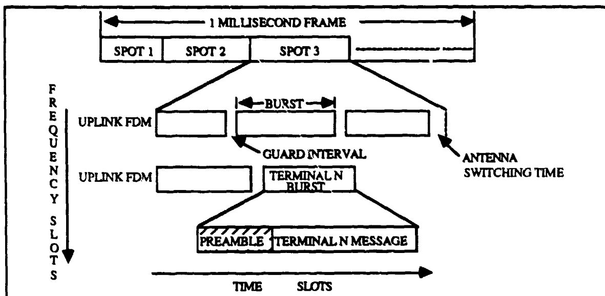
Figure 3.7 Uplink Beam FDM/TDM Organization [ Ref. 29: p. 673 ]
