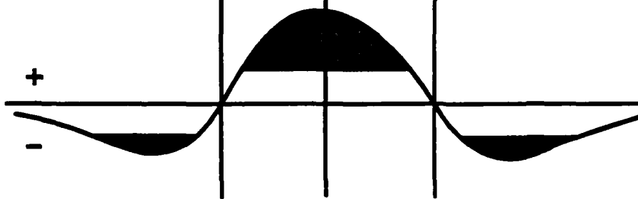
Figure II-1. Microburst surface divergence signatures.
