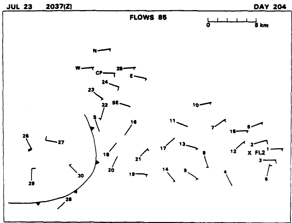
Figure IV-6. Mesonet plots showing the surface wind field for July 23, 1985 at 2035 and 2037 GMT. Full barb represents 5 m/s and half-barb 2.5 m/s.
