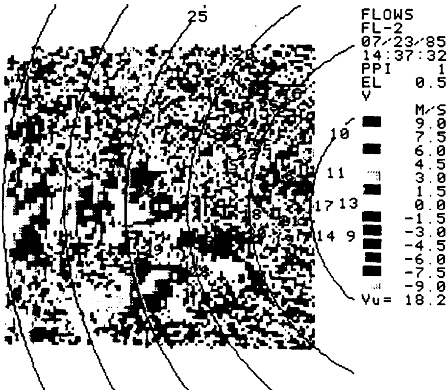
Figure IV-7. FL2 reflectivity and Doppler velocity fields for 23 July 1985 at \approx 1437 GMT (or \approx 2037 GMT). Elevation angle for both plots is 0.5^\circ . Range rings are every 5 km and locations of mesonet stations are overlaid.
