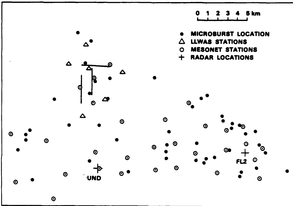
Figure III-1. Locations of the 1985 mesonet impacting microbursts.
