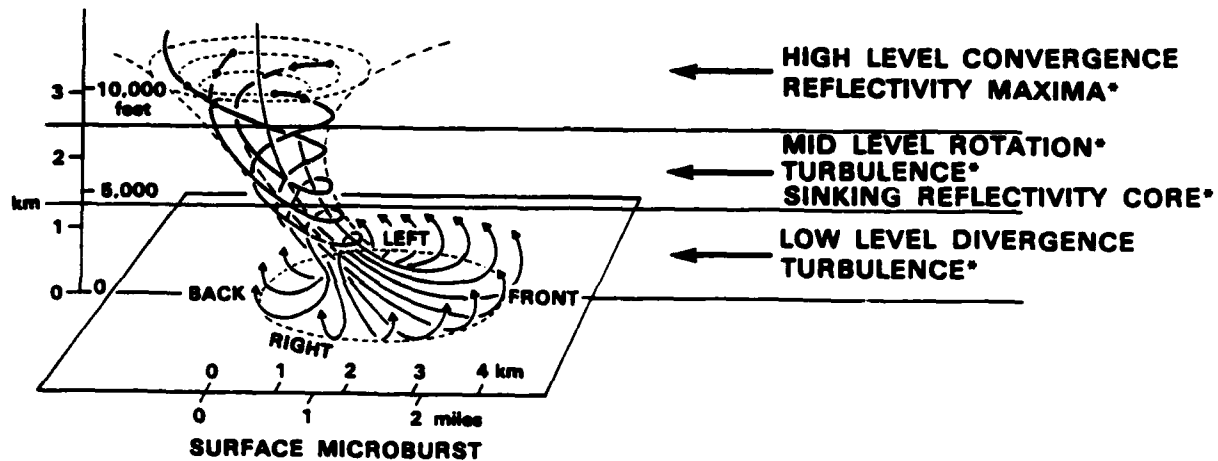
Figure II-2. Generalized model of a microburst.
