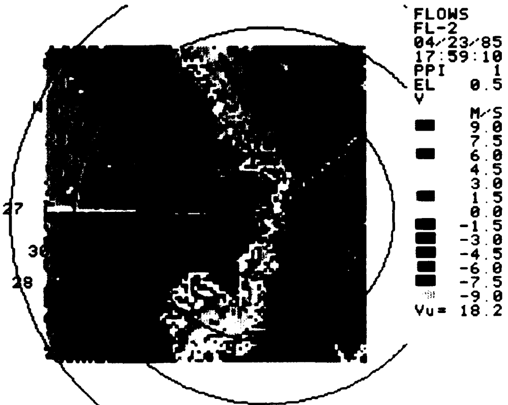
Figure IV-4. FL2 reflectivity and Doppler velocity fields for 23 April 1985 at \approx 1800 LST (or \approx 0000 GMT on 24 April 1985). Elevation angles for the reflectivity and velocity plots are 4^\circ and 0.5^\circ , respectively. Range rings are every 5 km and locations of mesonet stations are overlaid.
