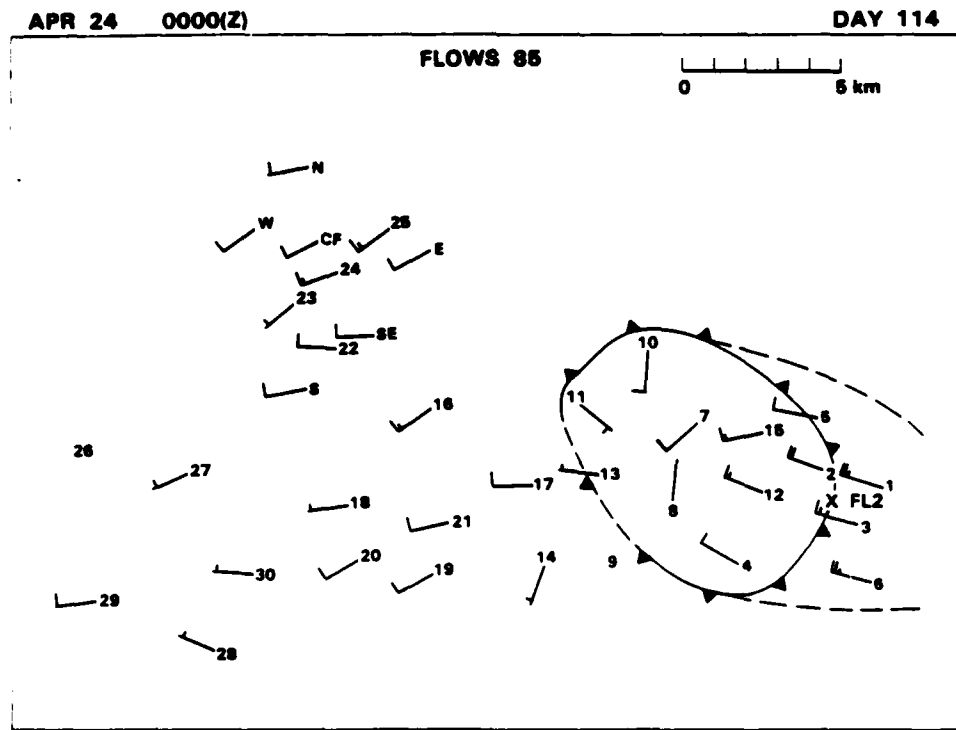
Figure IV-1. Mesonet plots showing the surface wind field for April 23, 1985 at 2358 (GMT) and April 24, 1985 at 0000 (GMT). Full barb represents 5 m/s and half-barb 2.5 m/s.
