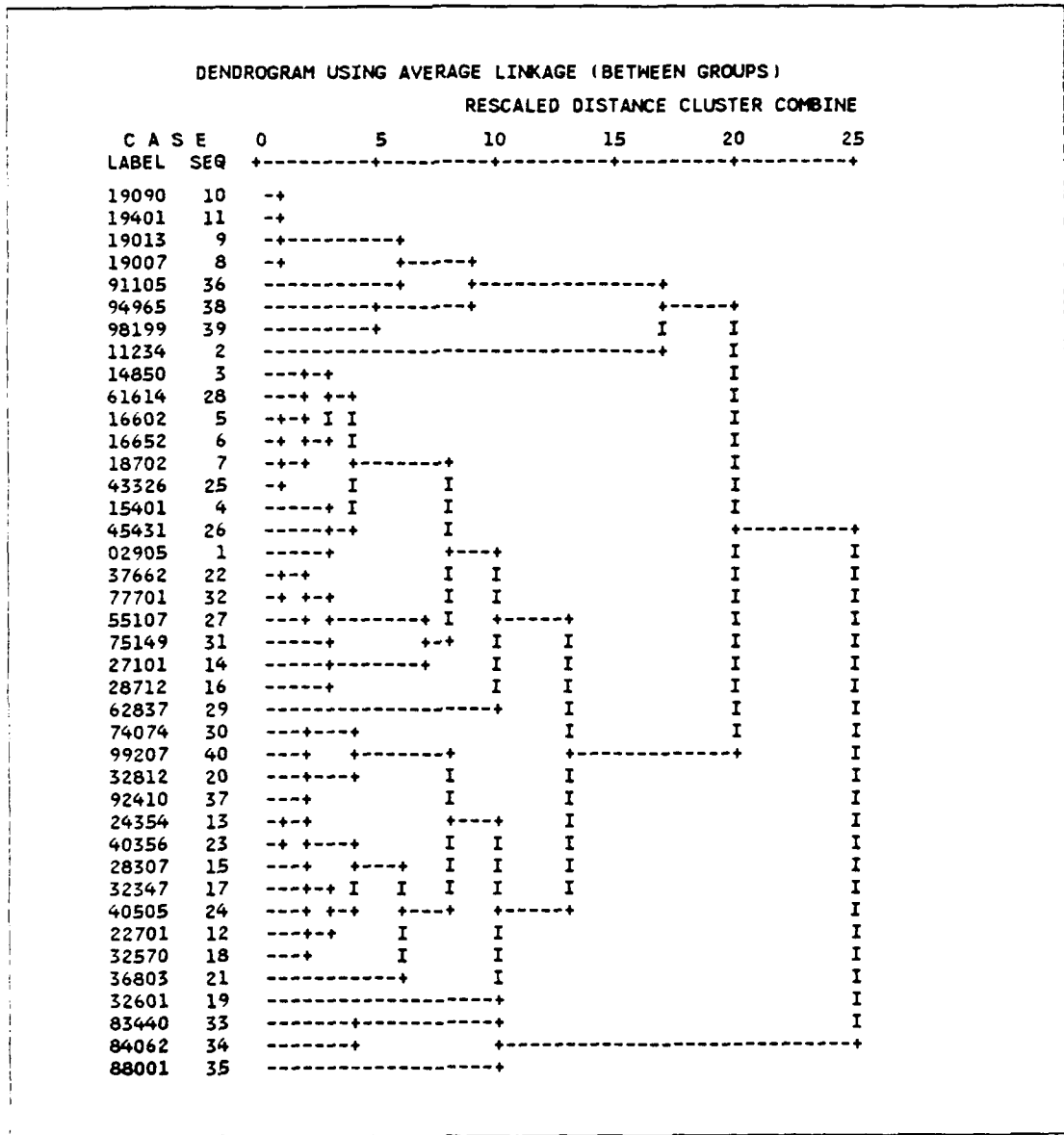
Figure 3.1 Accession Dendrogram.
