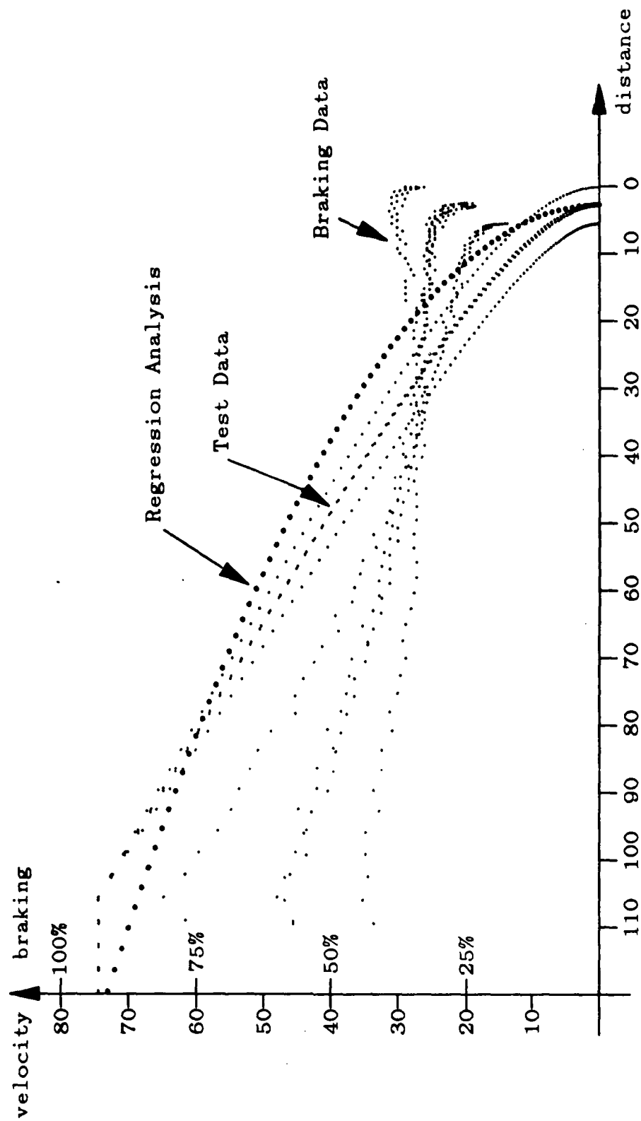
Figure 5.9 The "Super Driver" at 75 kmph.
