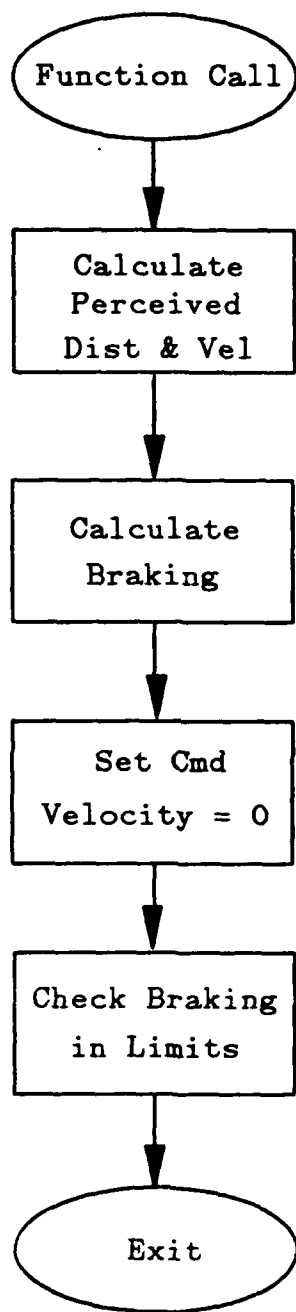
Figure 4.10 BRAKE.C Flowchart
