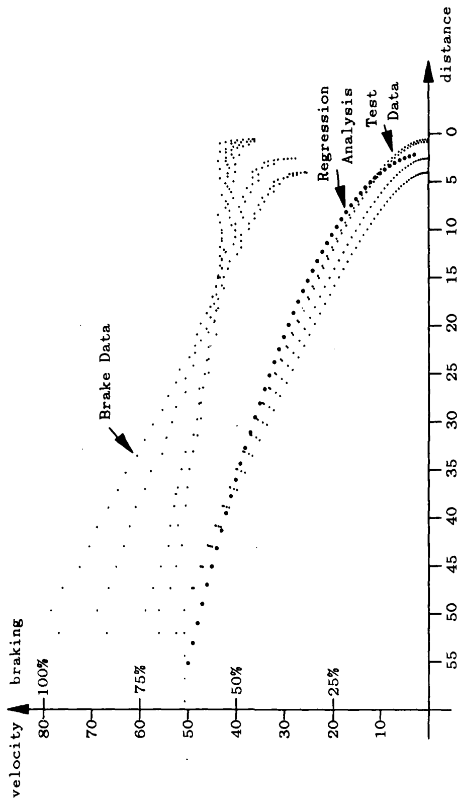
Figure 5.8 The "Super Driver" at 50 kmph.
