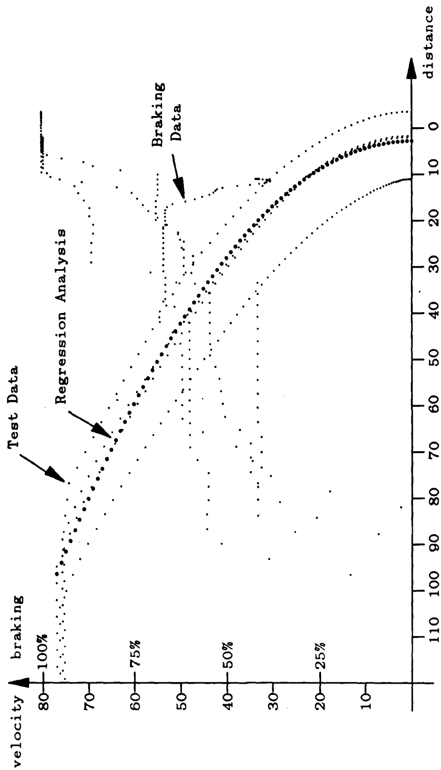
Figure 5.4 Four Trials by Driver #1, Alpha is 0.73.
