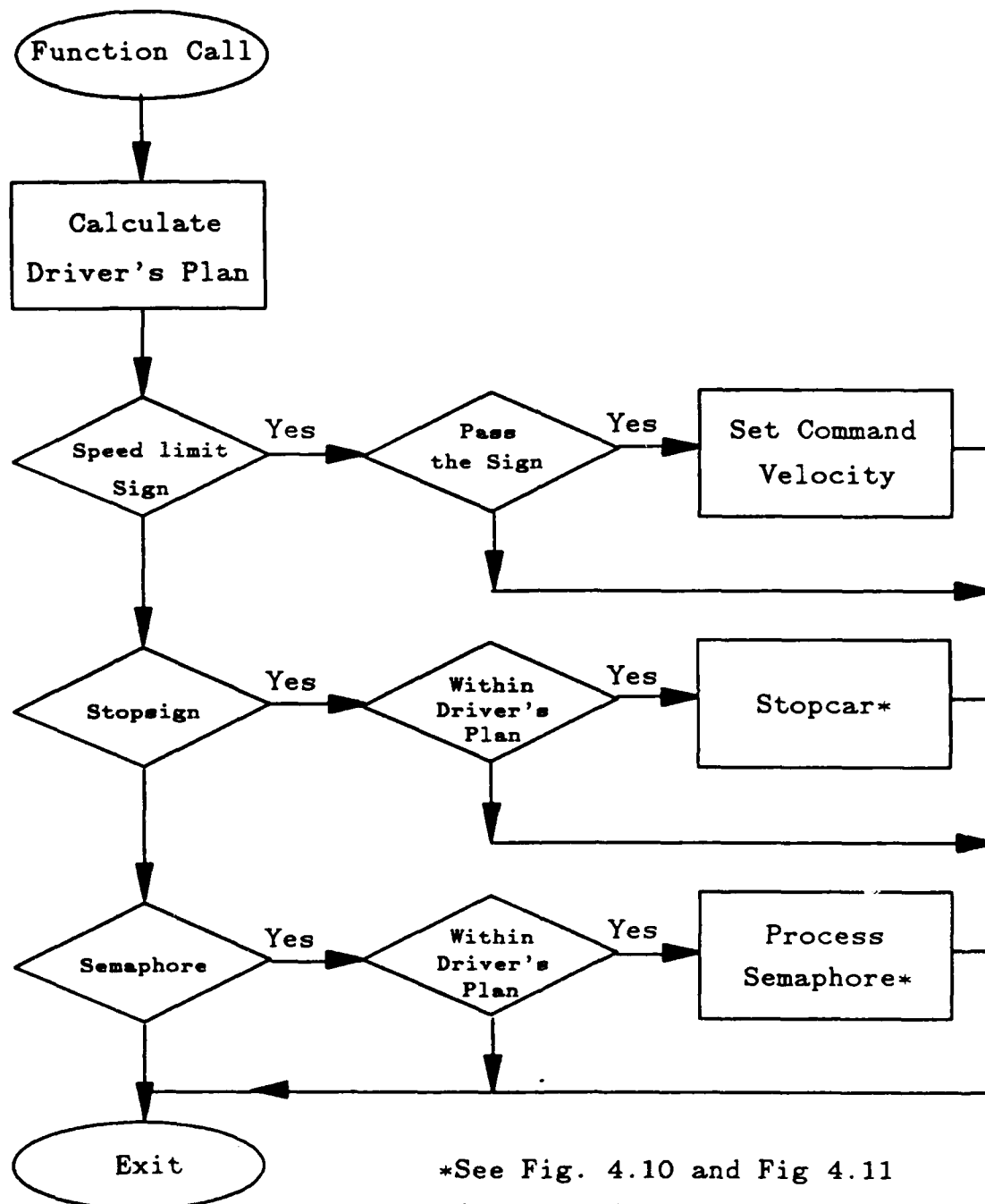
Figure 4.9 CRUISE.C flowchart
