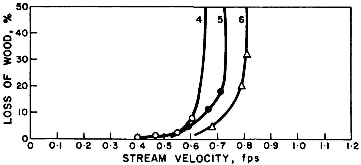
Fig. 21. Laboratory Tests of Flat Holding Booms
