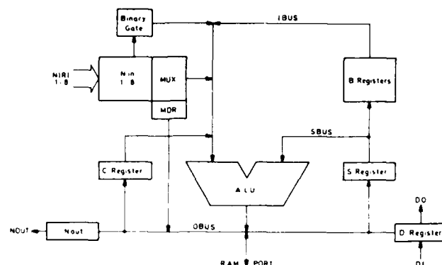
Figure 1. Data paths for the CLIP7 system.
