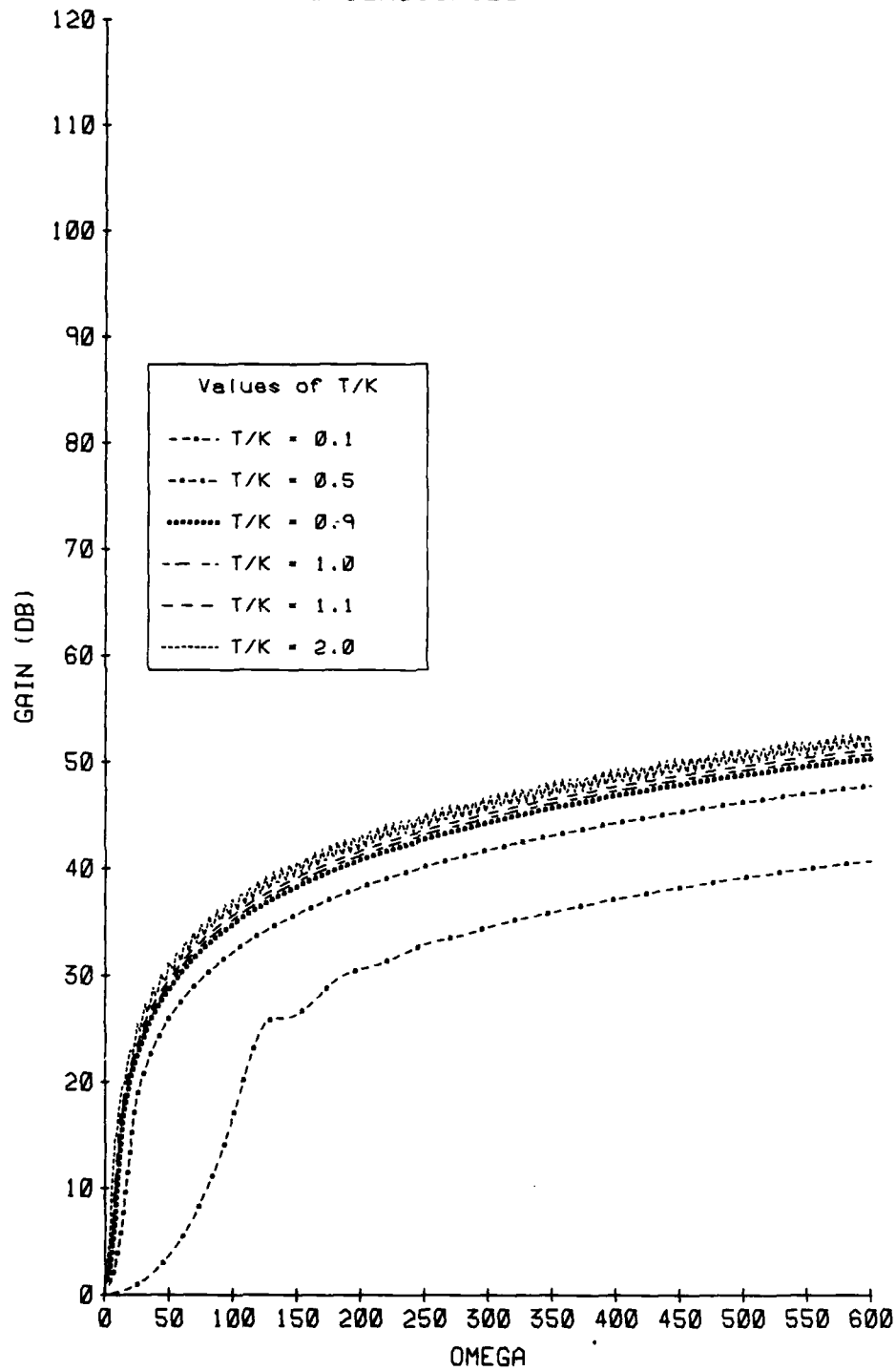
Figure 37(U) Gain for various T/K, Cos Shading and No Shaping, PFA = 10.**(-5)
