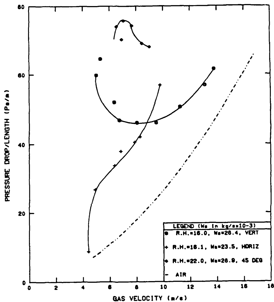
Figure A-22: Pressure Drop vs. Gas Velocity for 125µm Glass Beads for the Combined Orientations at the Higher Mass Flow Rate With Electrostatics
