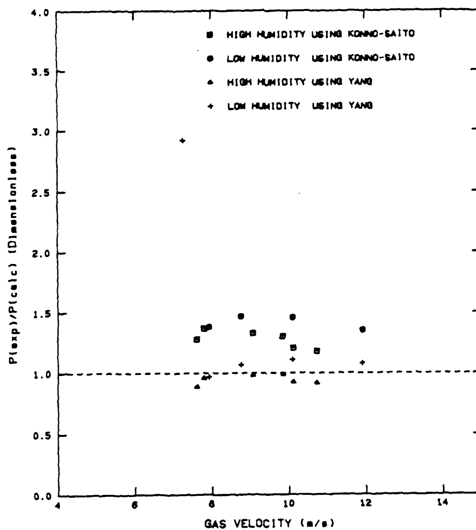
Figure A-56: Ratio of Experimental to Calculated Pressure Drop vs. Gas Velocity for 450 \mu m Glass Beads in the Horizontal Orientation with W = 30. \times 10^{-3}
