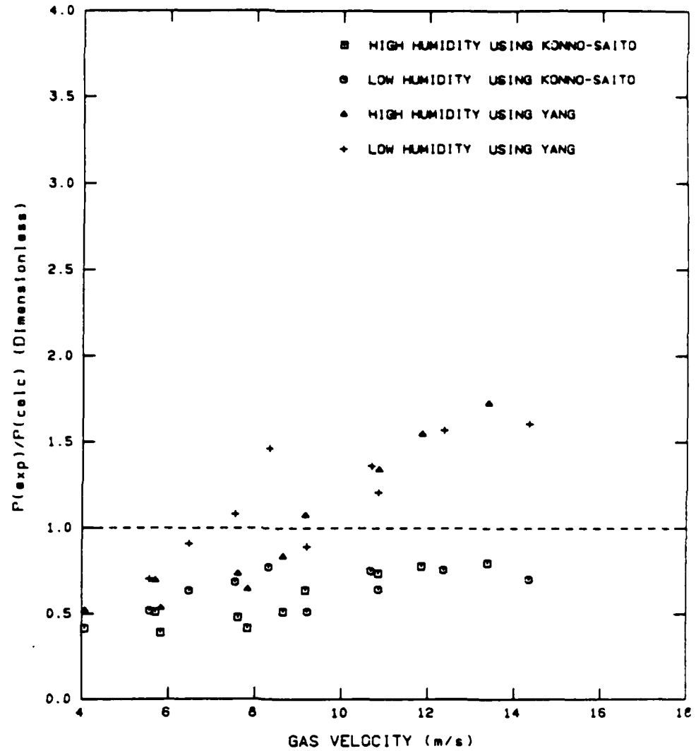
Figure A-41: Ratio of Experimental to Calculated Pressure Drop vs. Gas Velocity for 79 \mu\text{m} Glass Beads in the Vertical Orientation with W_s \approx 18 \times 10^{-3}
