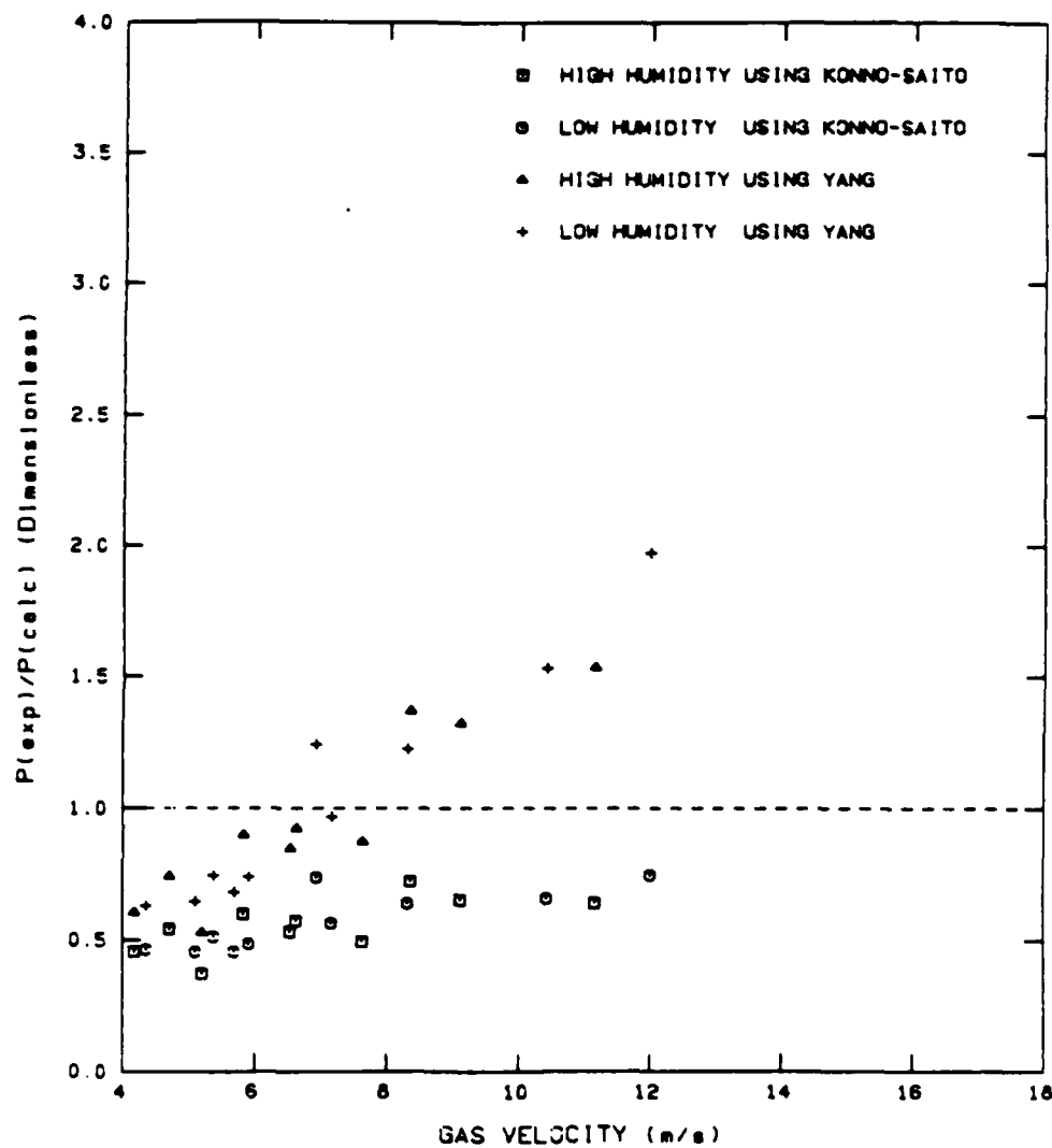
Figure A-40: Ratio of Experimental to Calculated Pressure Drop vs. Gas Velocity for 79 \mu\text{m} Glass Beads in the Vertical Orientation with W_i = 9. \times 10^{-3}
