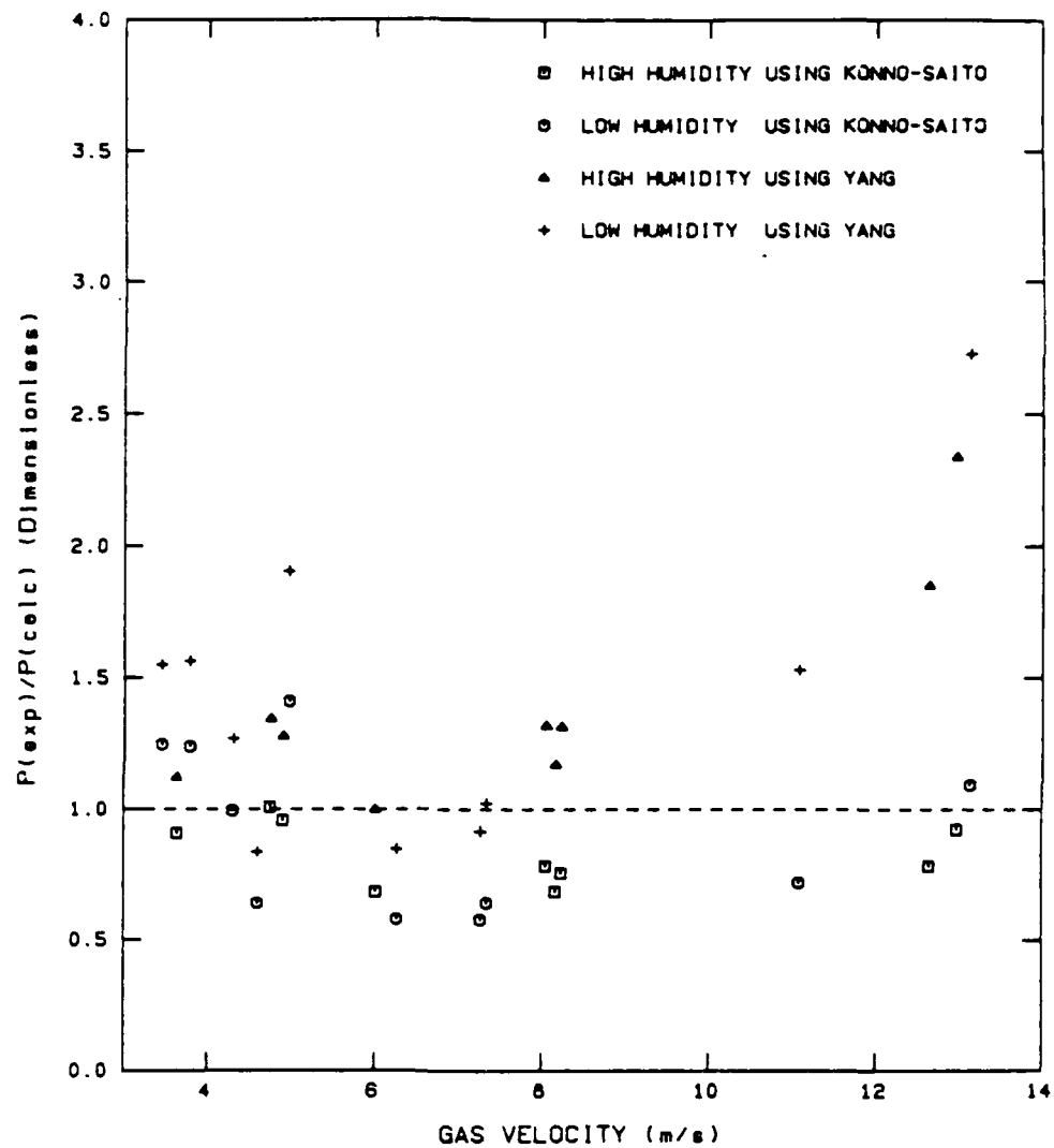
Figure A-50: Ratio of Experimental to Calculated Pressure Drop vs. Gas Velocity for 128 \mu m Plexiglas Beads in the Vertical Orientation with W_s = 12 \cdot 10^{-3}
