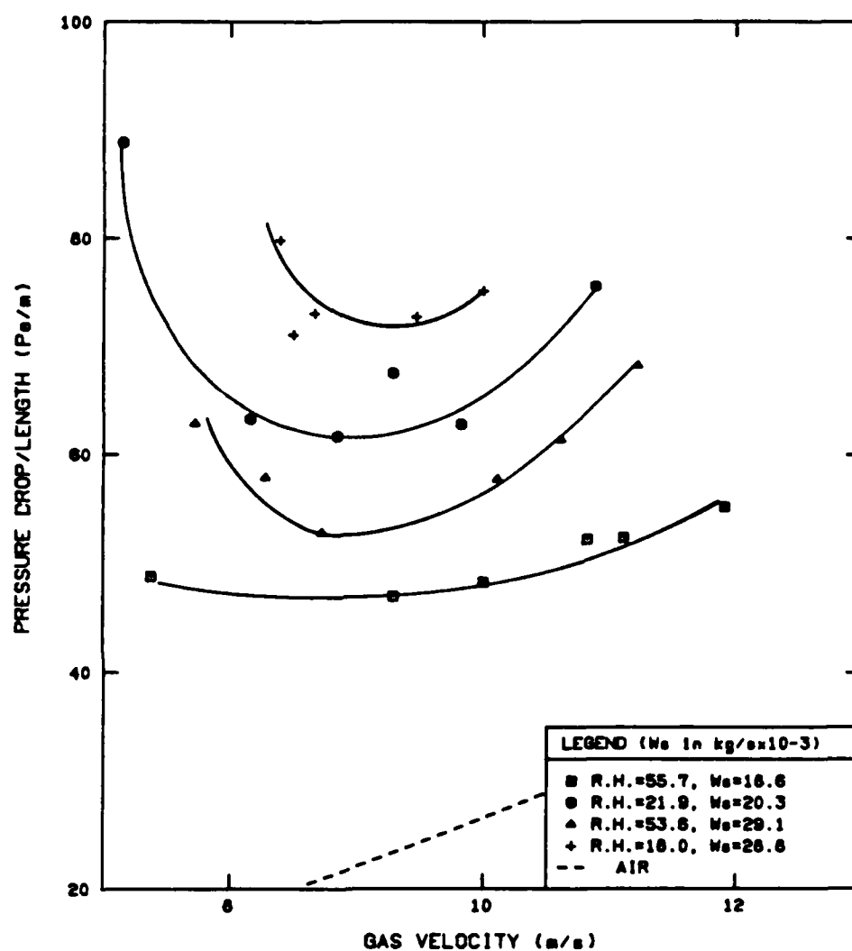
Figure A-14: Pressure Drop vs. Gas Velocity for the 450µm Glass Beads in the Inclined Orientation
