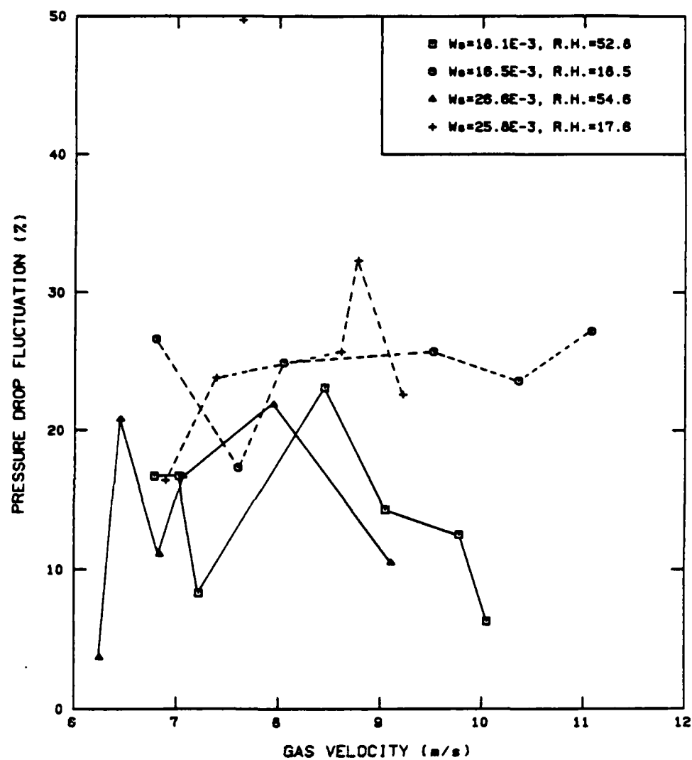
Figure A-35: Pressure Drop Fluctuation vs. Gas Velocity for 79µm Glass Beads in the Inclined Orientation
