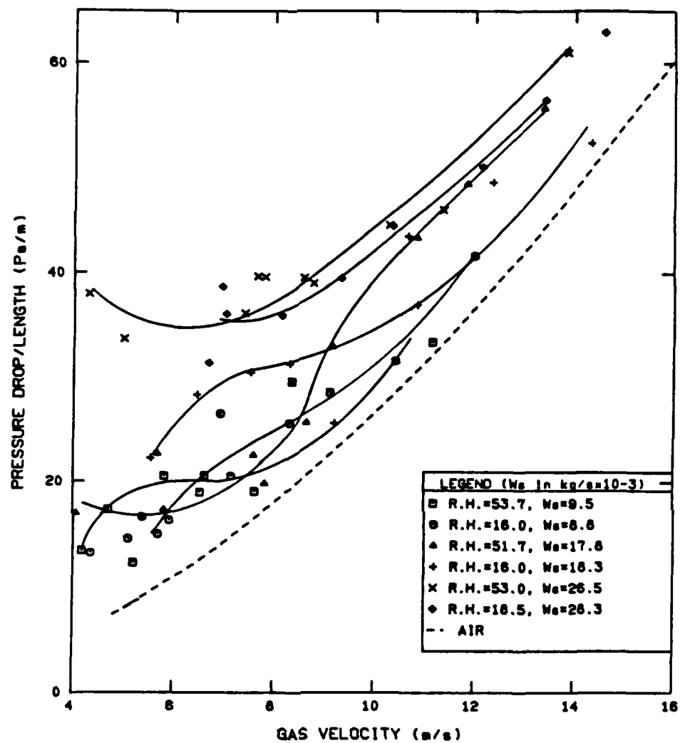
Figure A-8: Pressure Drop vs. Gas Velocity for 79µm Glass Beads in the Vertical Orientation
