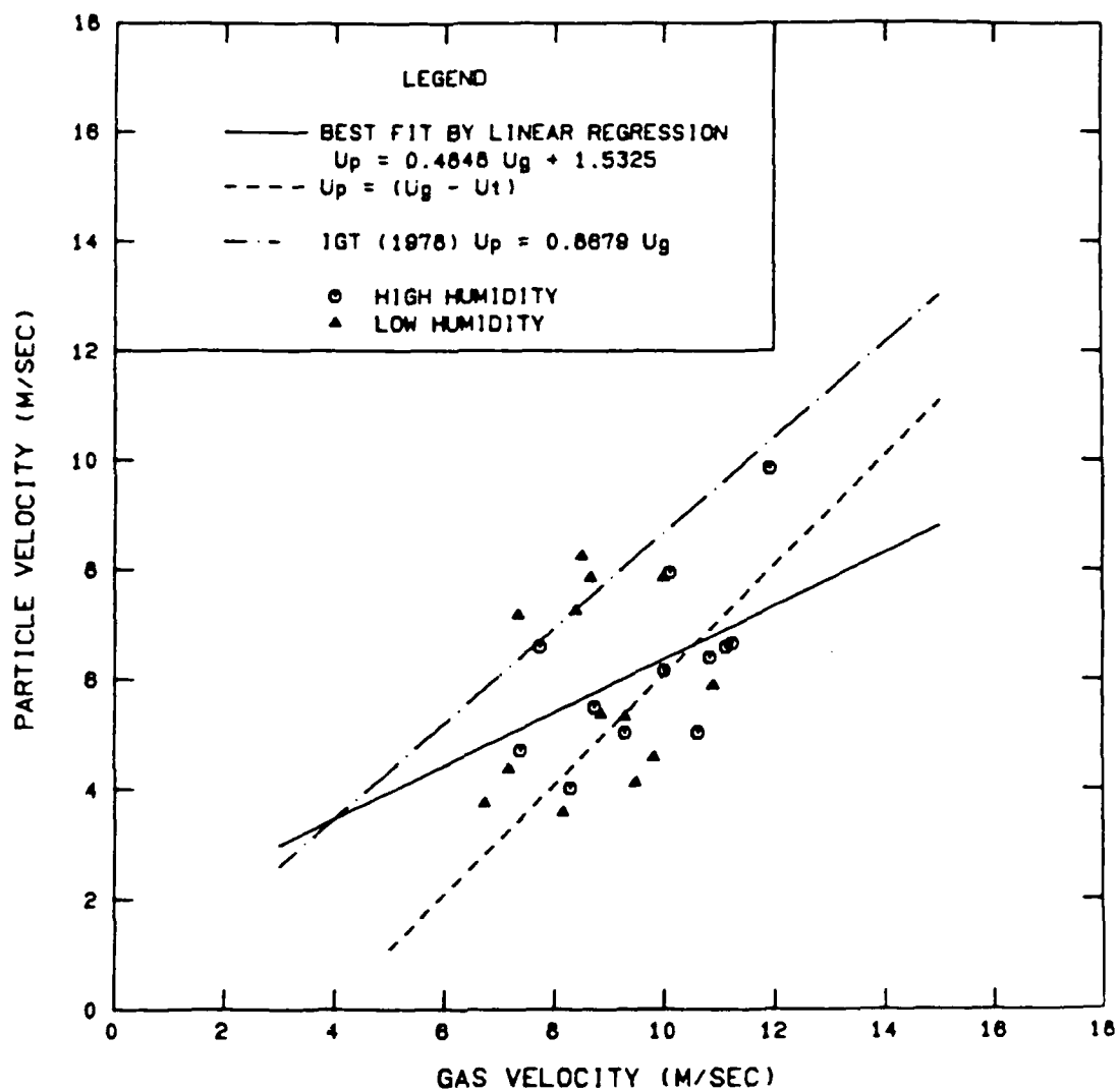
Figure A-7: Particle Velocity vs. Gas Velocity for 450 \mu m Glass Beads in the Inclined Orientation
