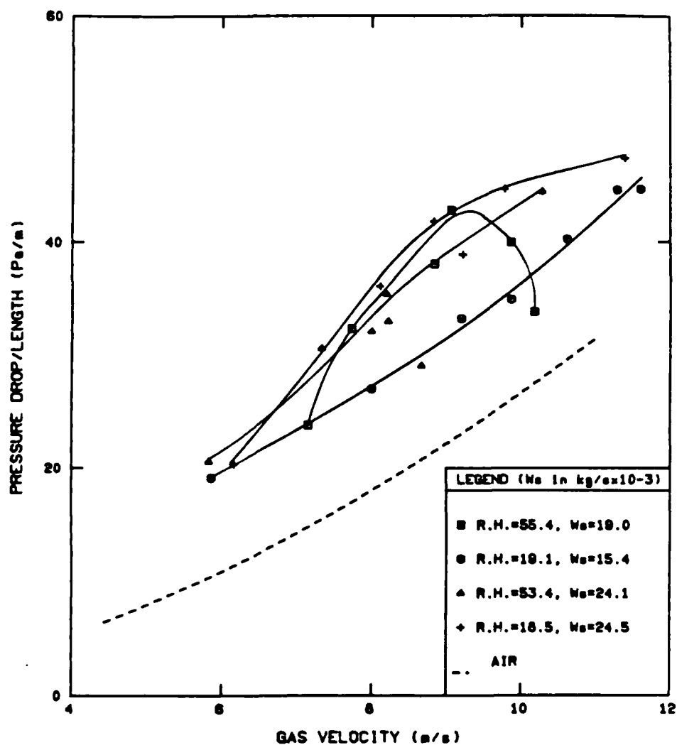
Figure A-11: Pressure Drop vs. Gas Velocity for 79μm Glass Beads in the Horizontal Orientation
