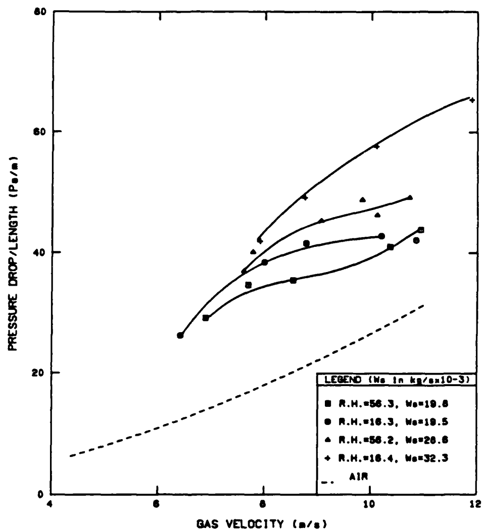
Figure A-12: Pressure Drop vs. Gas Velocity for 450µm Glass Beads in the Horizontal Orientation
