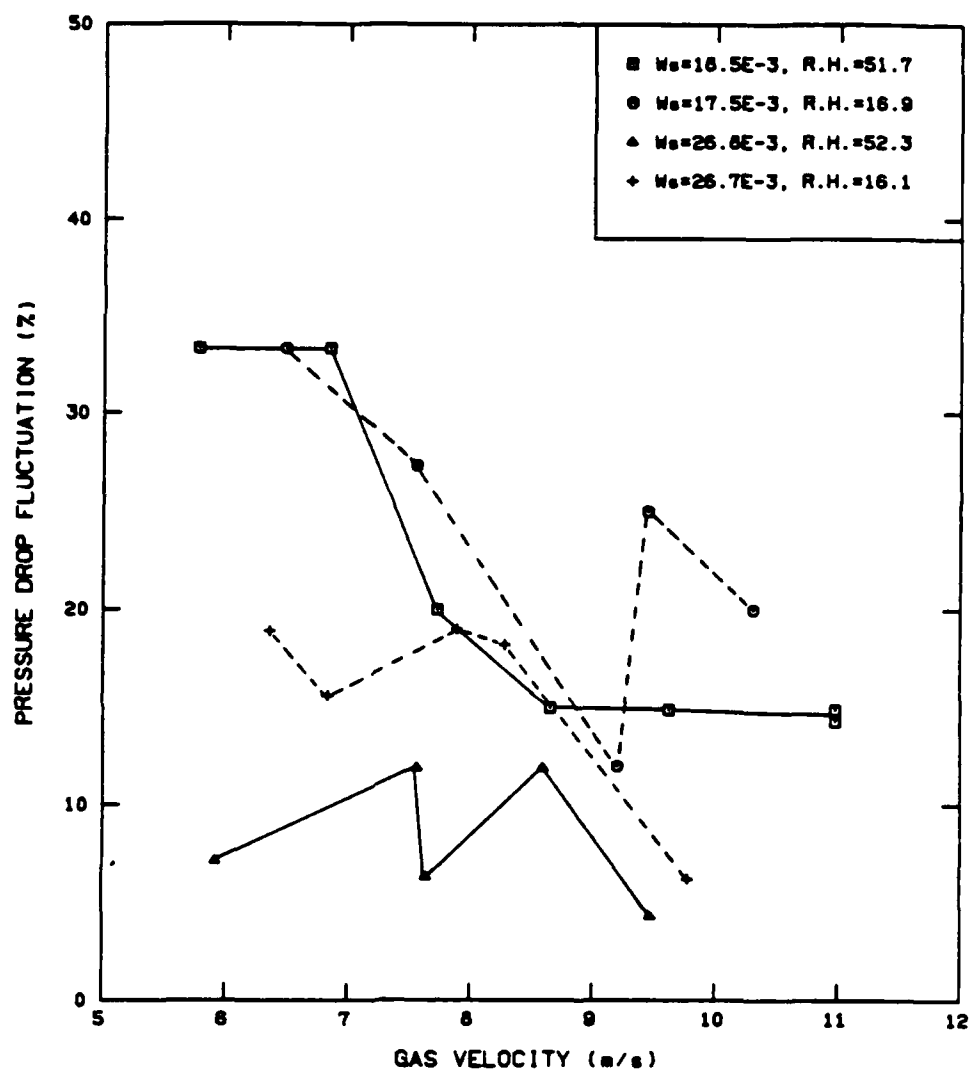
Figure A-31: Pressure Drop Fluctuation vs. Gas Velocity for 125µm Glass Beads in the Horizontal Orientation
