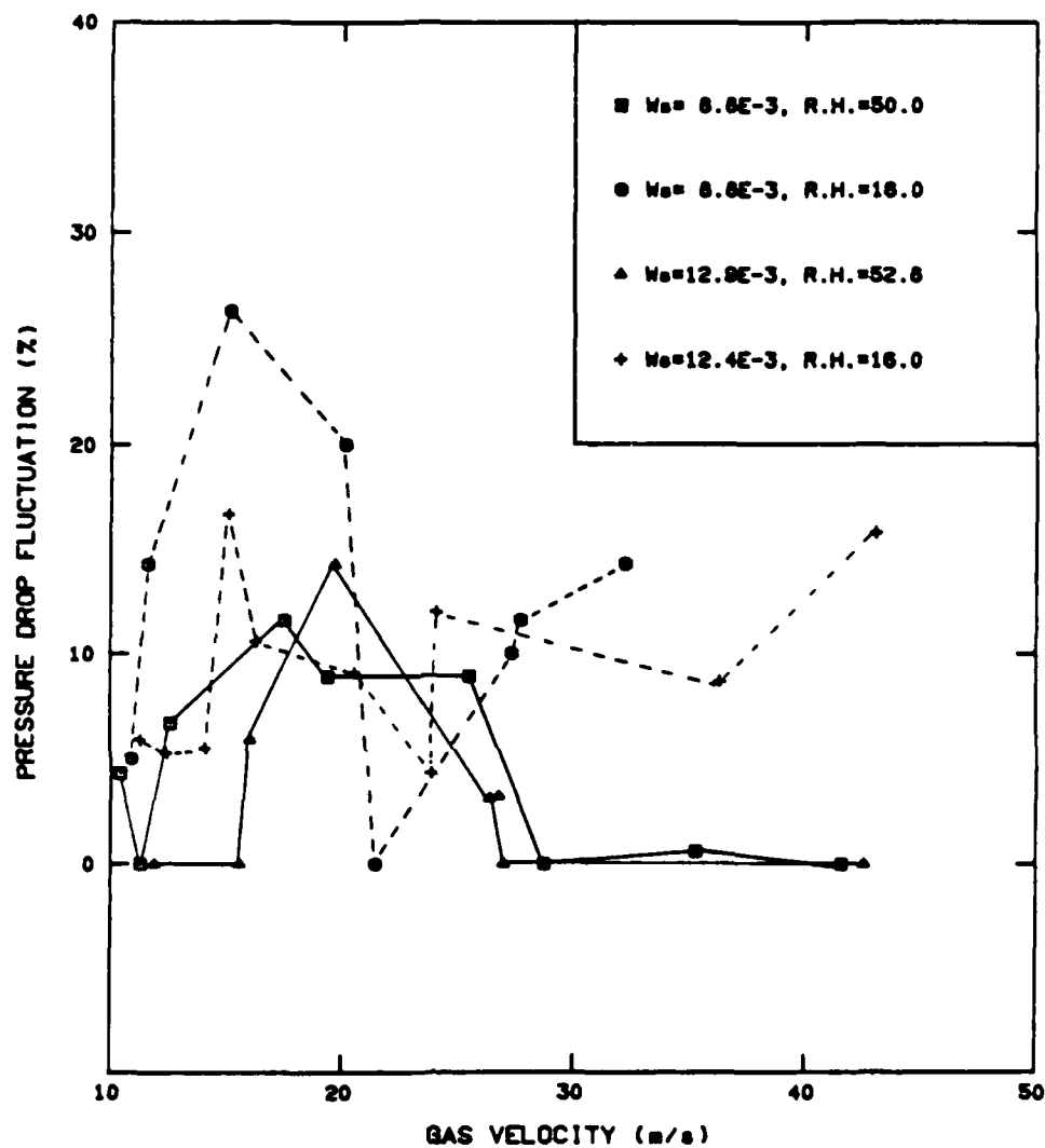
Figure A-30: Pressure Drop Fluctuation vs. Gas Velocity for 128µm Plexiglas Beads in the Vertical Orientation
