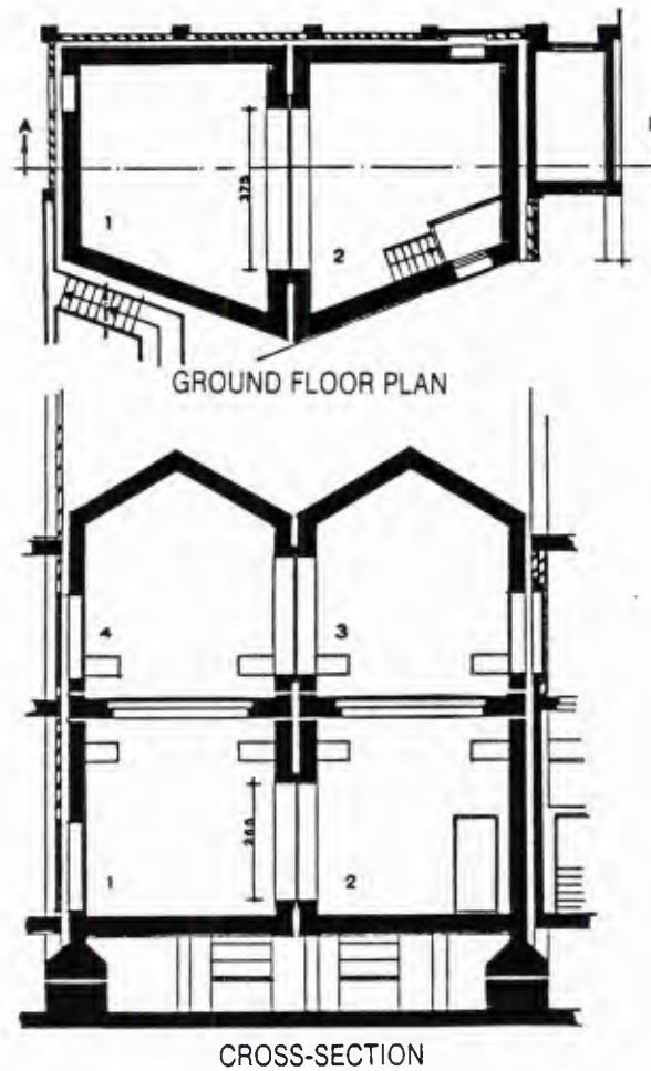
Figure 4-17. TH Acoustic Isolation Rooms
