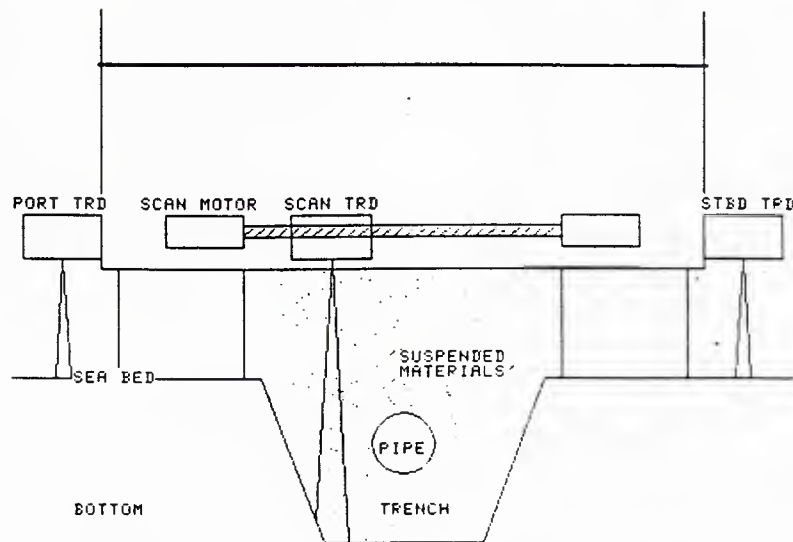
Figure 2-18(b). Diagram of Trench Scanner
