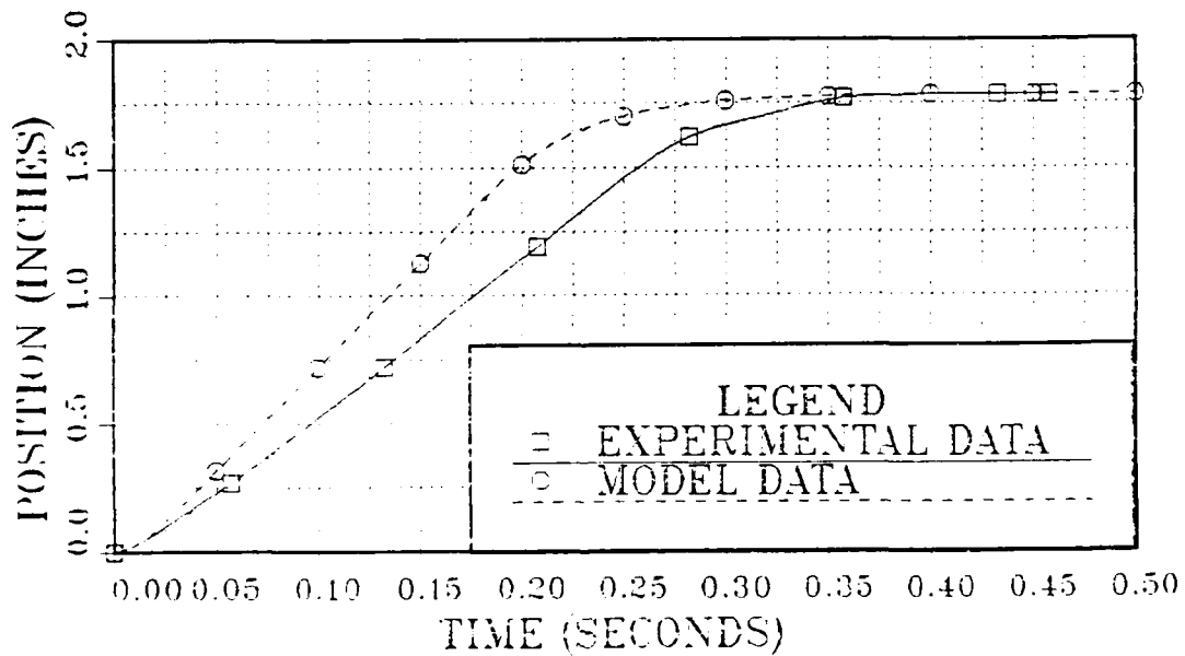
Figure 2.8 Analog Step Step Response (1.785 in.).
