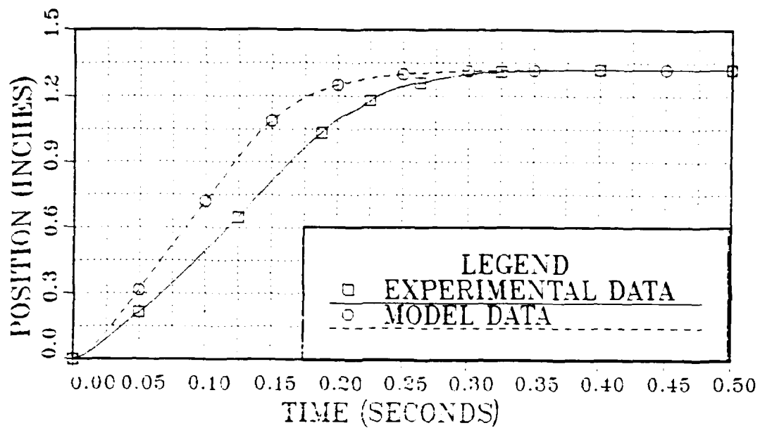
Figure B.5 Analog System Step Response (1.32 in.).
