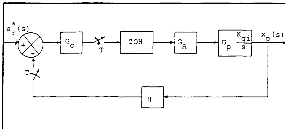
Figure 3.3 Digital System Model.
