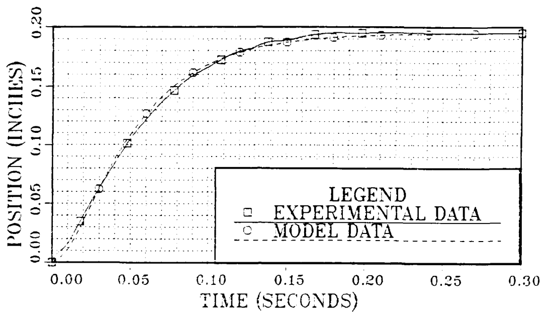
Figure 2.7 Analog System Step Response (0.195 in.).
