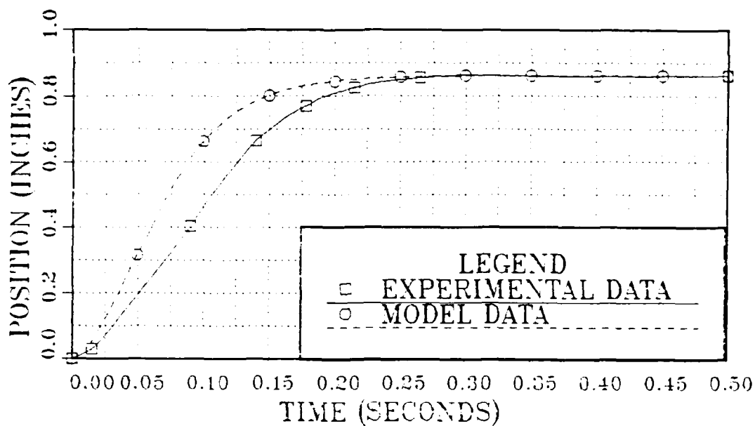
Figure B.3 Analog System Step Response (0.8625 in.).
