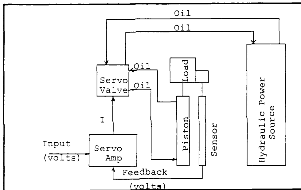
Figure 2.1 Analog System.
