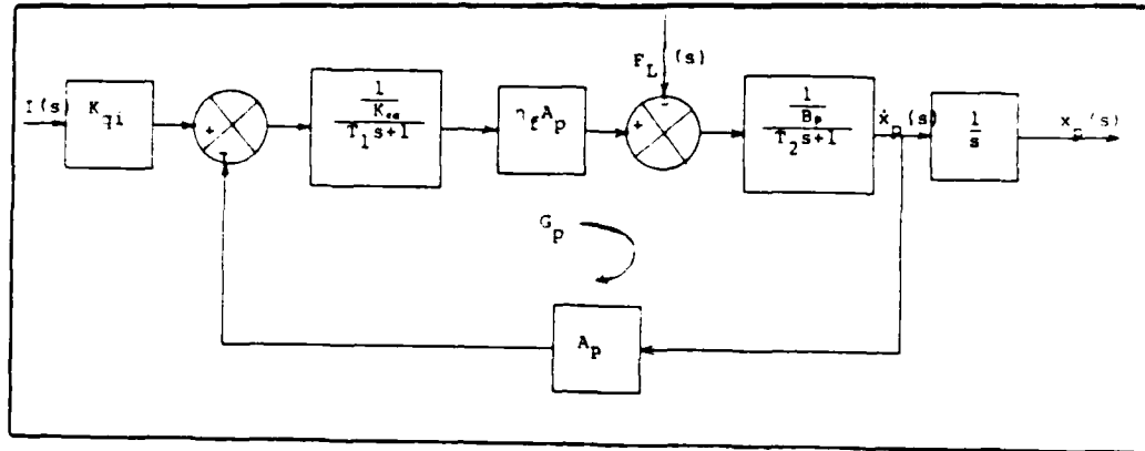
Figure 2.4 Analog System Block Diagram.
