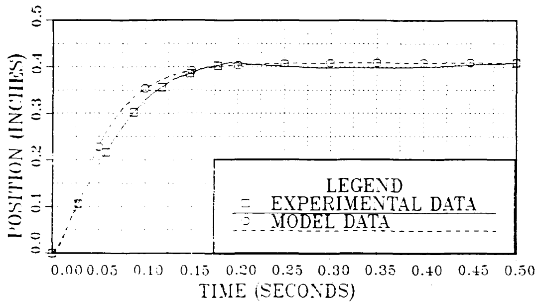
Figure B.1 Analog System Step Response (0.4088 in.).
