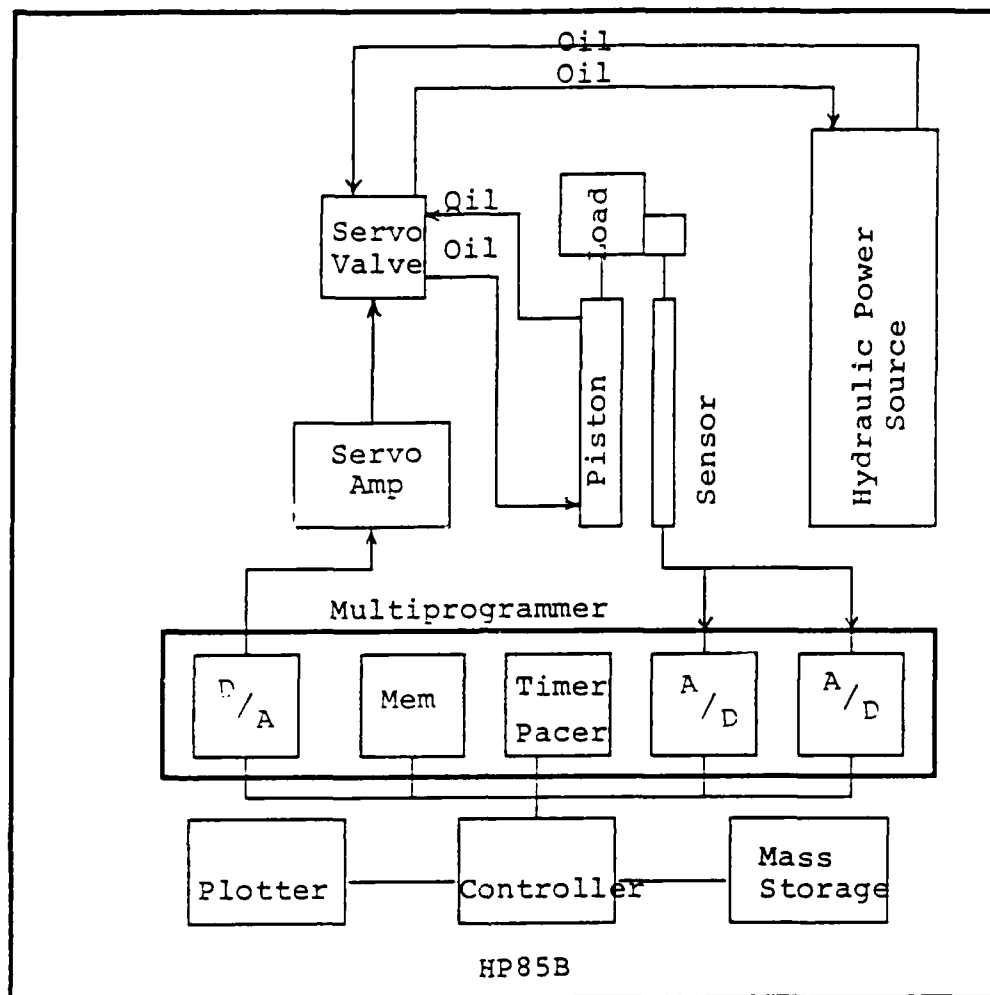
Figure 3.1 System with Digital Controller.
