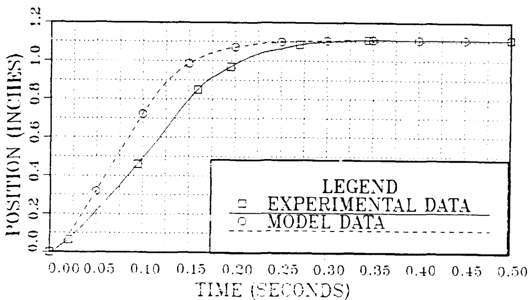
Figure B.4 Analog System Step Response (1.11 in.).
