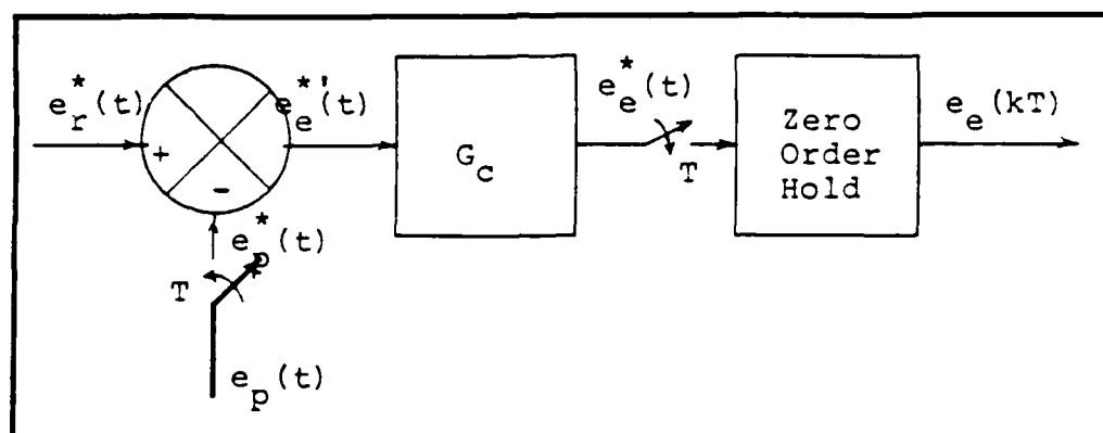
Figure 3.2 Microcomputer Controller.
