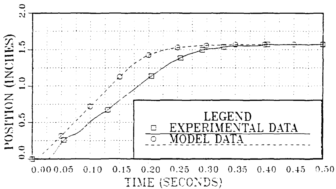
Figure B.6 Analog System Step Response (1.57 in.).
