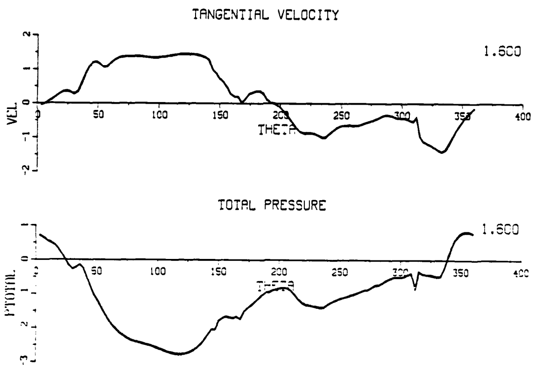
Figure A.6 Position of vortices, velocity and pressure distribution at T^* = 1.600 .
