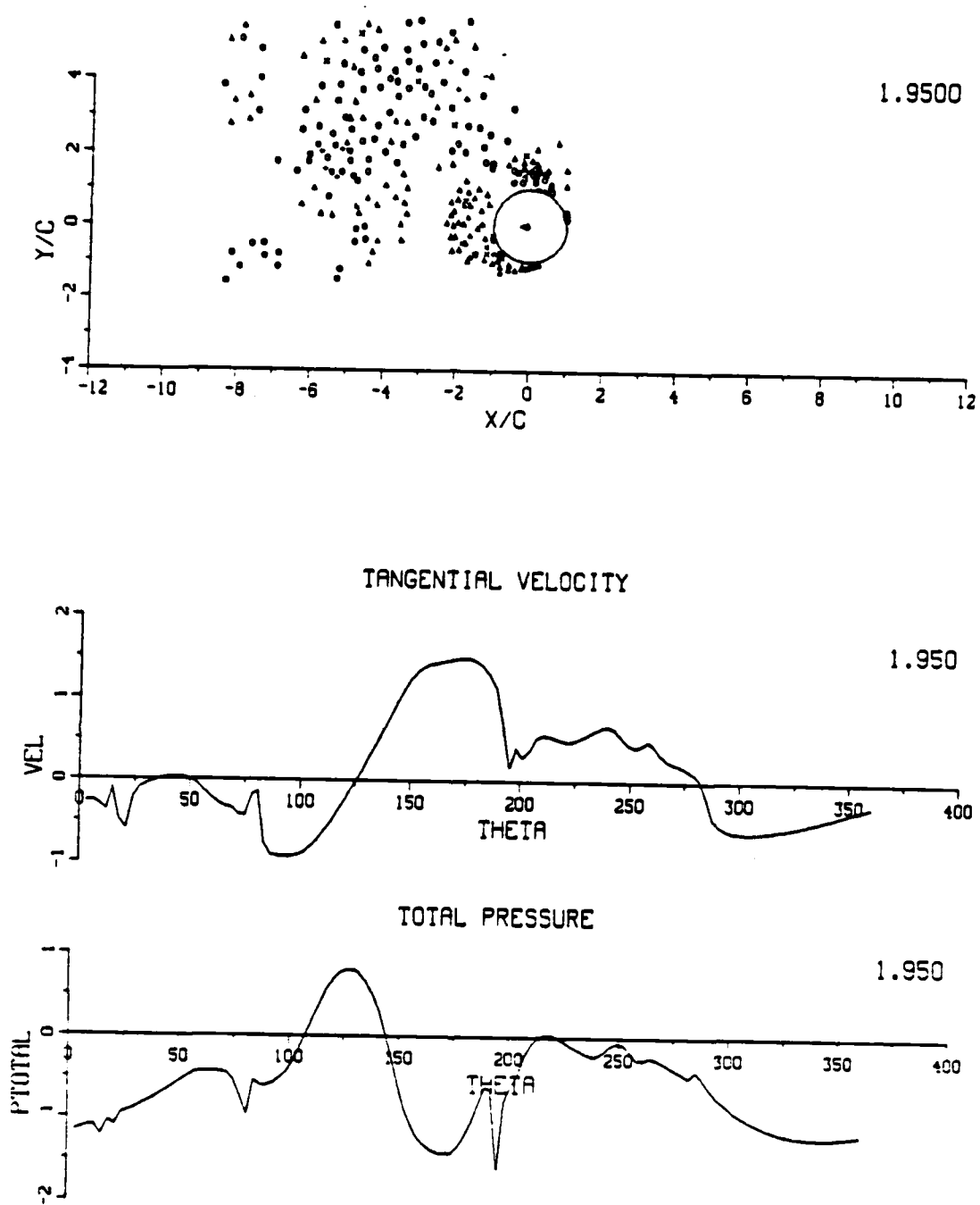
Figure A.10 Position of vortices, velocity and pressure distribution at T^* = 1.950 .
