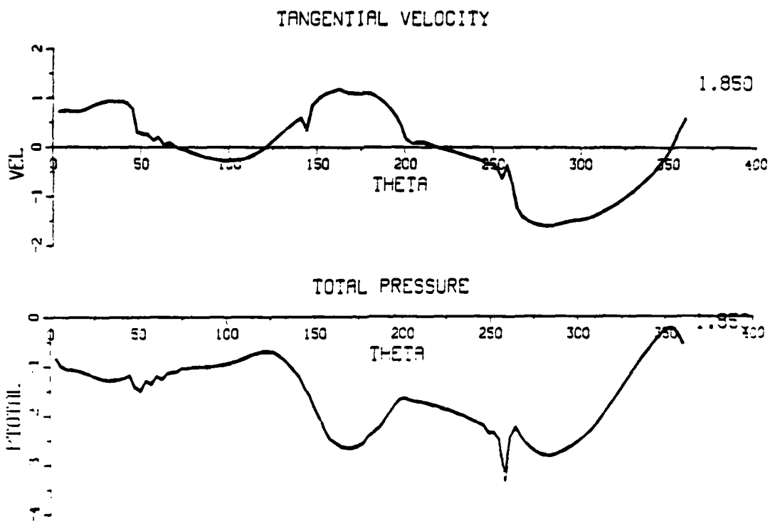
Figure A.9 Position of vortices, velocity and pressure distribution at T^* = 1.850 .
