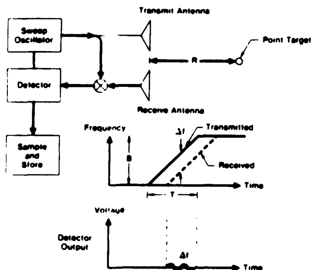
Figure 2.2. The Linear-FM Imaging Systems and Waveforms
