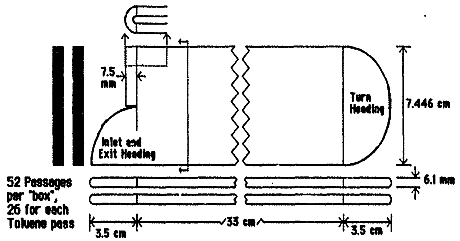
Figure 18 - Toluene Passage Dimensions and Heading
