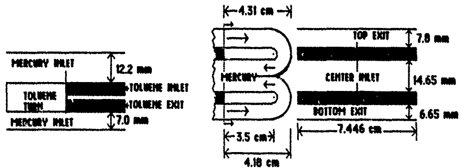
Figure 19 - Mercury Passage Dimensions
