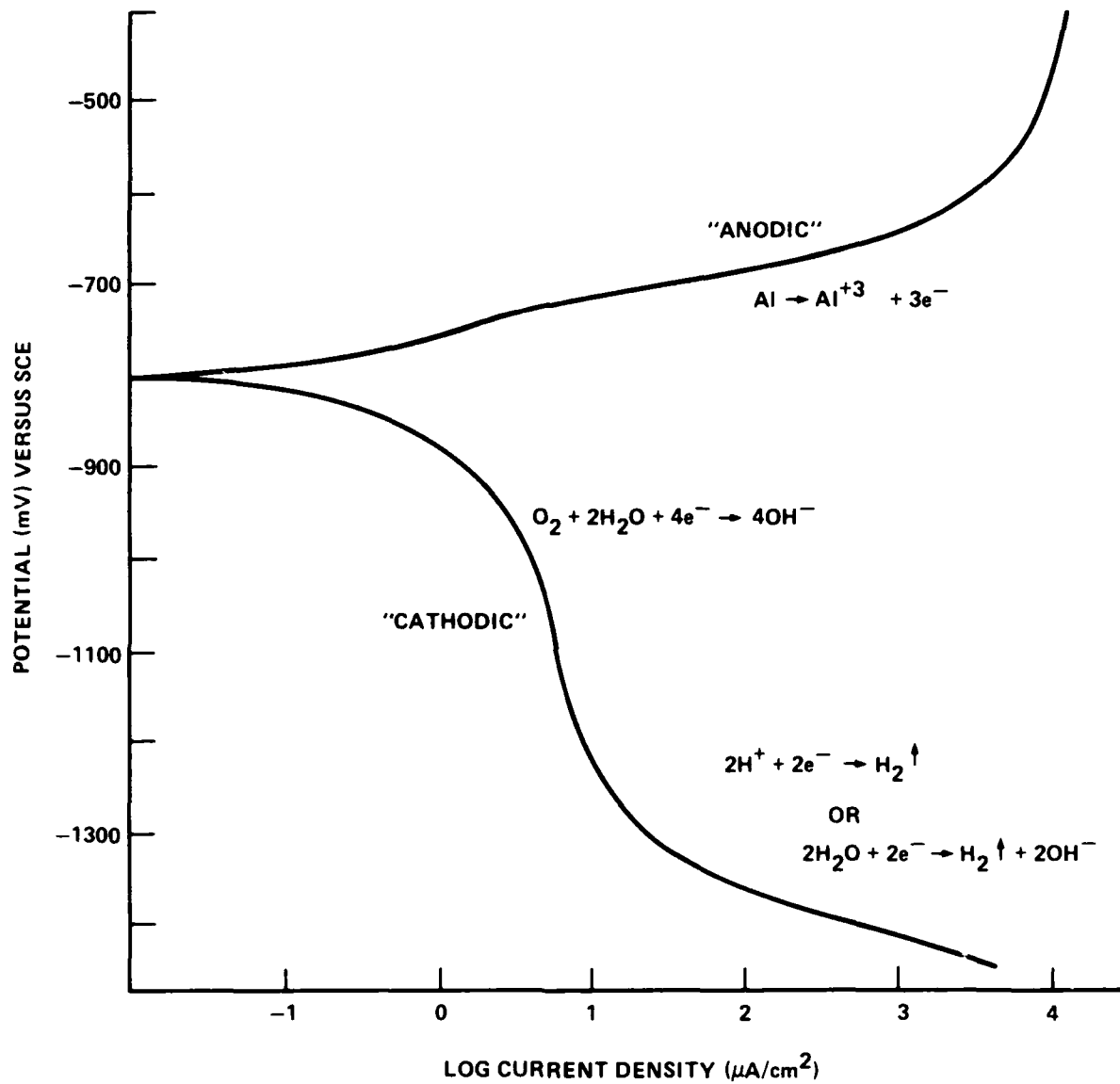
FIGURE 3. EXAMPLES OF POTENTIODYNAMIC POLARIZATION CURVES, INCLUDING TYPICAL ANODIC AND CATHODIC ELECTRODE REACTIONS
