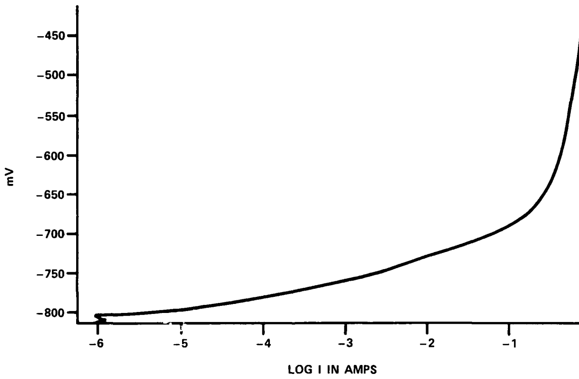
FIGURE 8. POTENTIODYNAMIC ANODIC POLARIZATION CURVE FOR IN-9052 EXPOSED TO 3.5% NaCl
