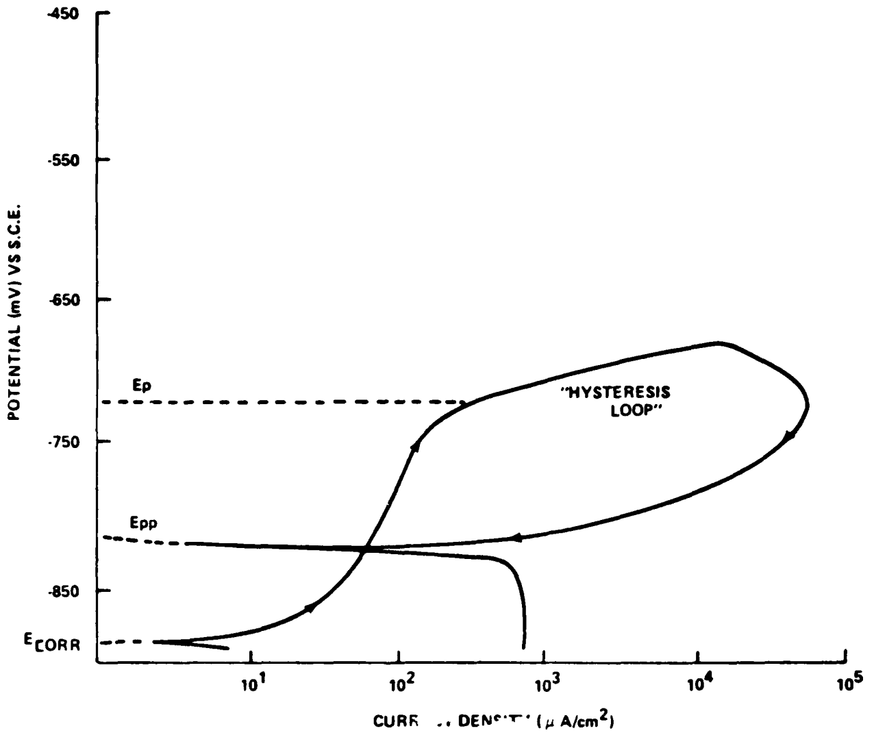
FIGURE 4. POTENTIODYNAMIC PITT SCAN FOR AN ALUMINUM COMPOSITE IN 3% NaCl
