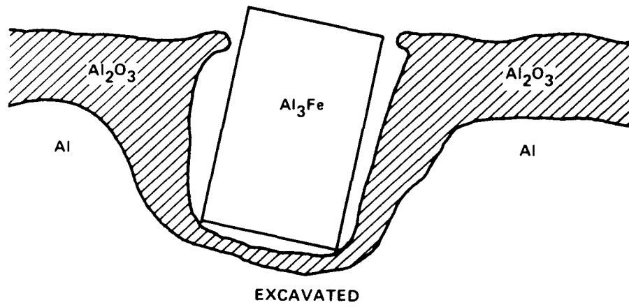
FIGURE 38*. SCHEMATIC OF Al_3Fe PARTICLE EXCAVATED BY PITTING AT ITS MARGINS
