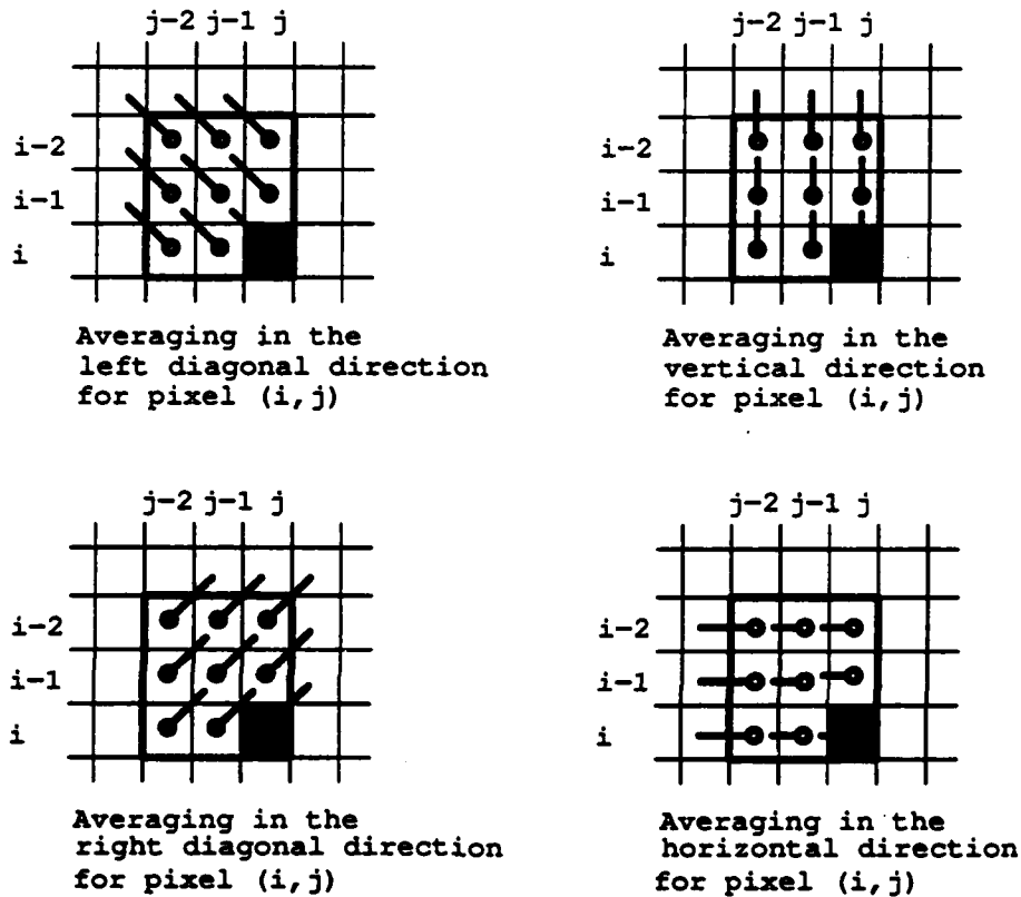
Figure 5-2: Calculation of the interest operator
