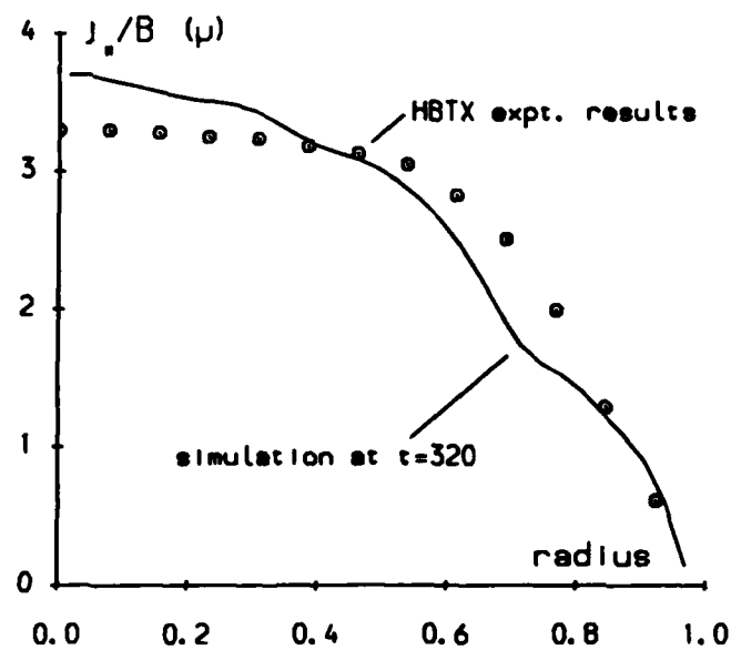
Fig.5 j_1/B vs. radius and heuristic comparison with experiment. (Case: S = 10^3 , \eta = \text{flat} ).
