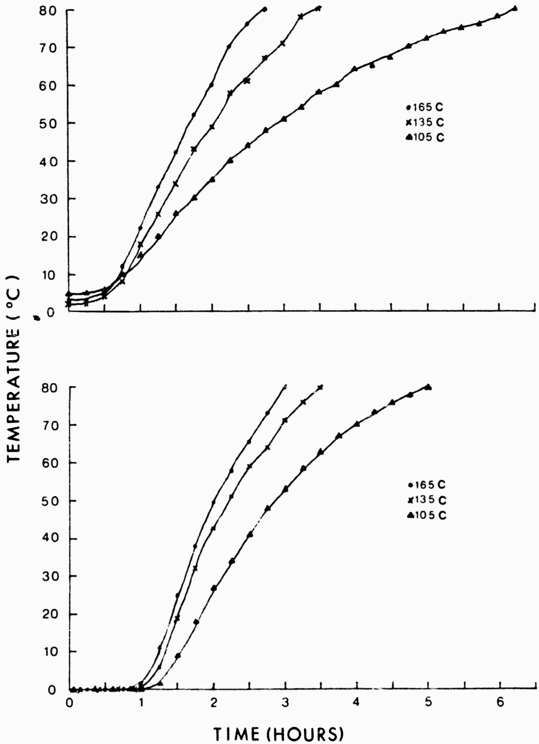
Figure 3. Representative Heating Curves for One Turkey Roast Cooked in a Home Convection Oven (above) and Two Turkey Roasts Cooked in an Institutional Convection Oven (below).
