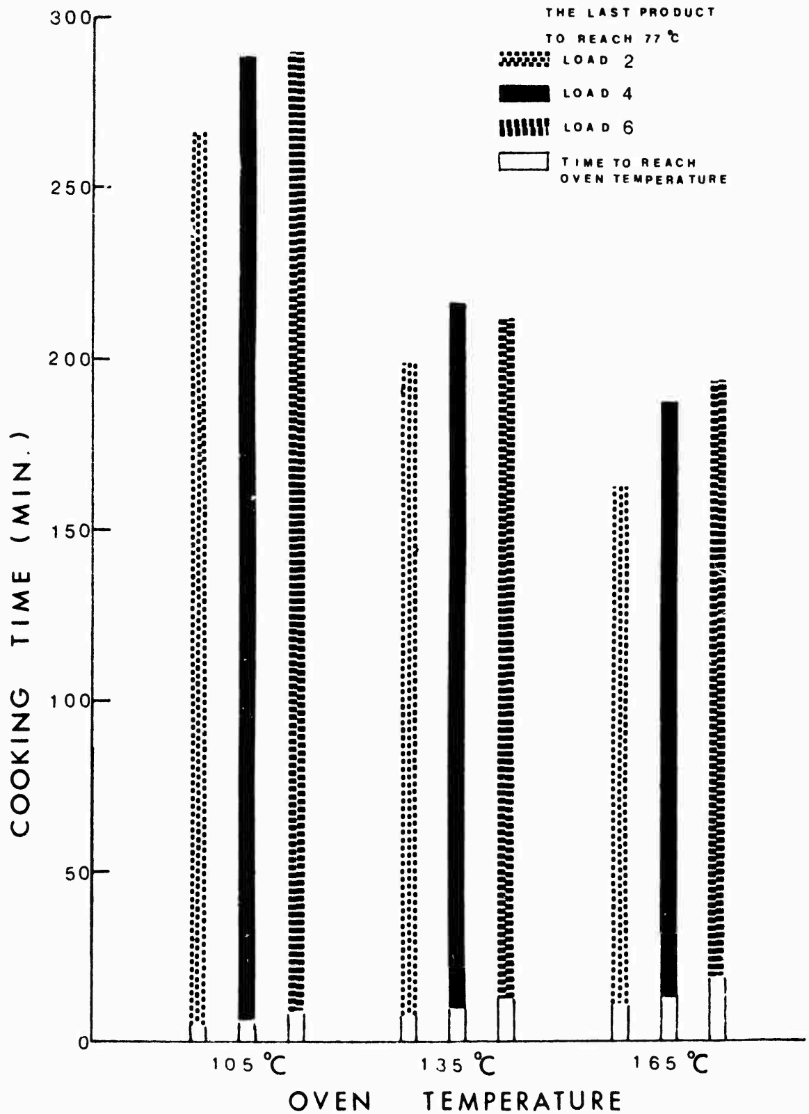
Figure 4. Time Needed to Reach Predetermined Oven Temperatures and Total Cooking Times for All Turkey Rolls to Reach 77°C or above in a Convection Oven When Using Three Oven Loads and Three Oven Temperatures.
