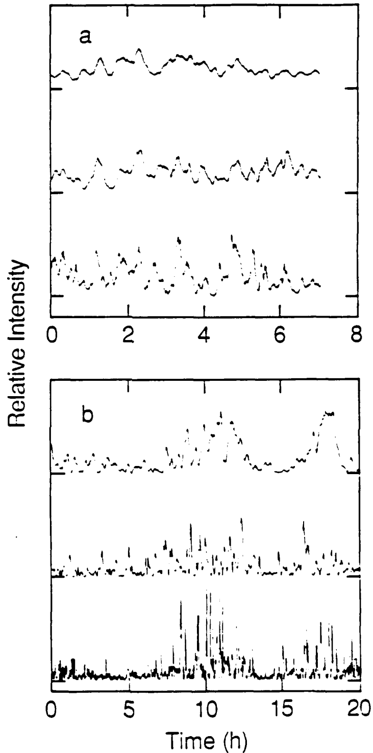
FIG. 2. (a) The intensity series at 2.8 km. The interval between tick marks is 5 times the mean intensity. The series are for 750 Hz (top trace), 1500 Hz (middle trace), and 2800 Hz (bottom trace). (b) 20 hours of intensity data for three frequencies over the 35-km path. The interval between tick marks is 10 times the mean intensity. The acoustic frequencies are 410 Hz (top), 1010 Hz (middle) and 4671 Hz (bottom).
