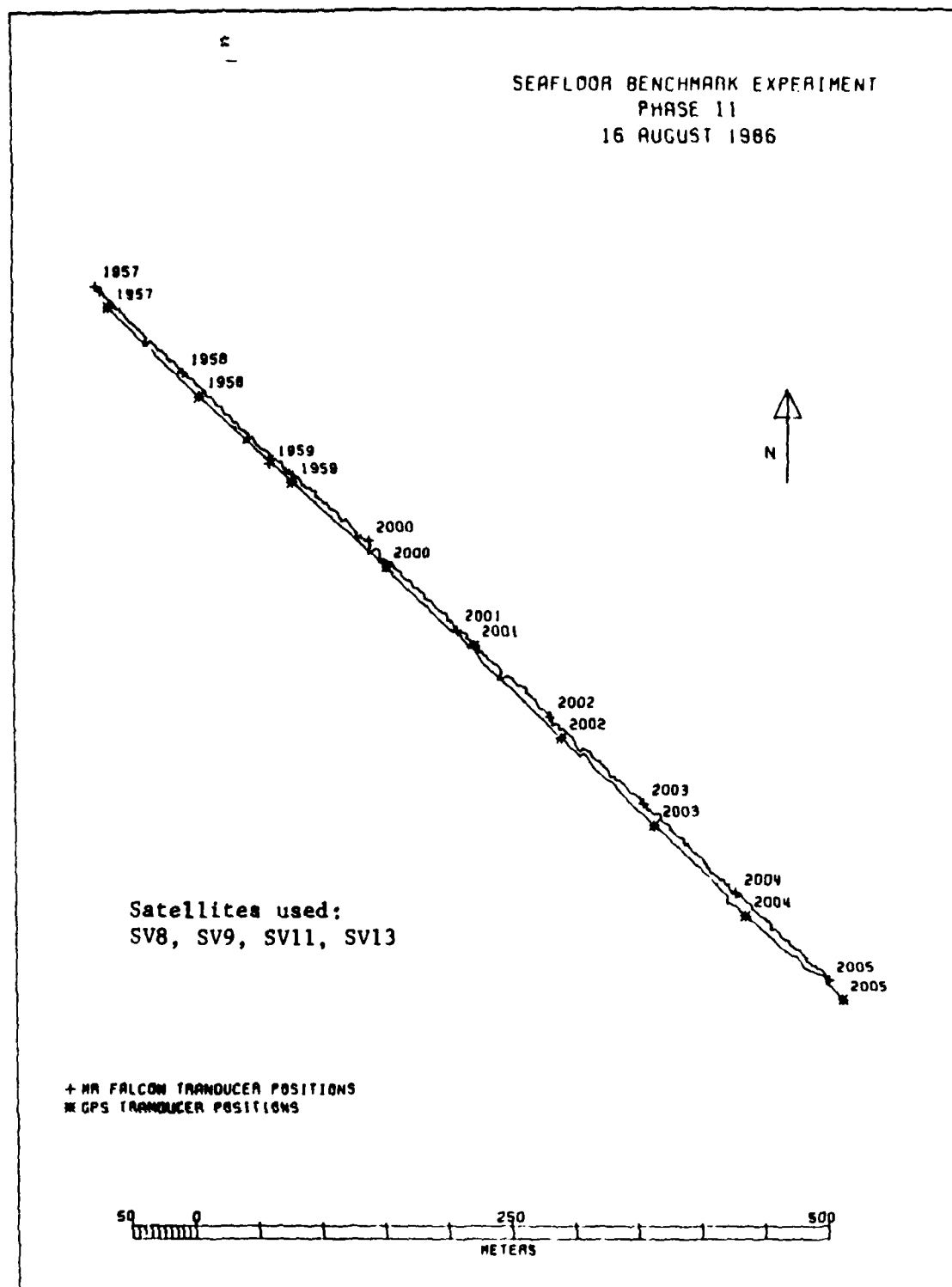
Figure 4.9 Period 7 (Case B). Constraining to geoidal height.
