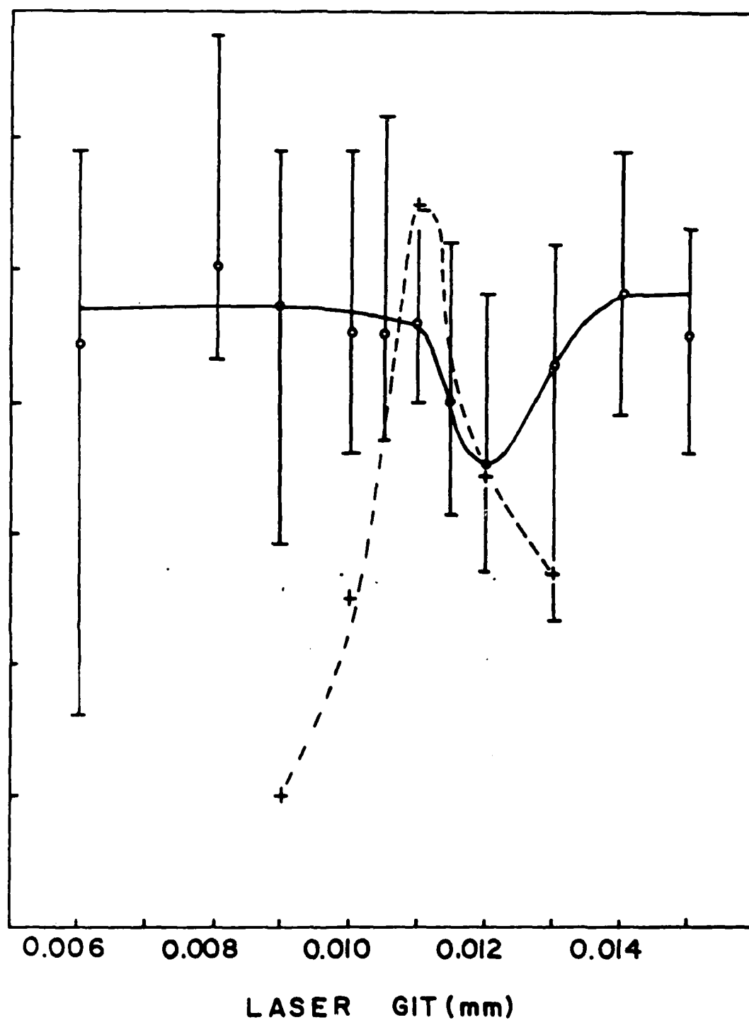
Figure 31. Laser transmission intensity (o) in 665-Pa neon discharge as the laser wavelength is tuned through 585.2-nm line. (The LIF intensity for similar conditions is shown by the crosses and dashed lines.)
