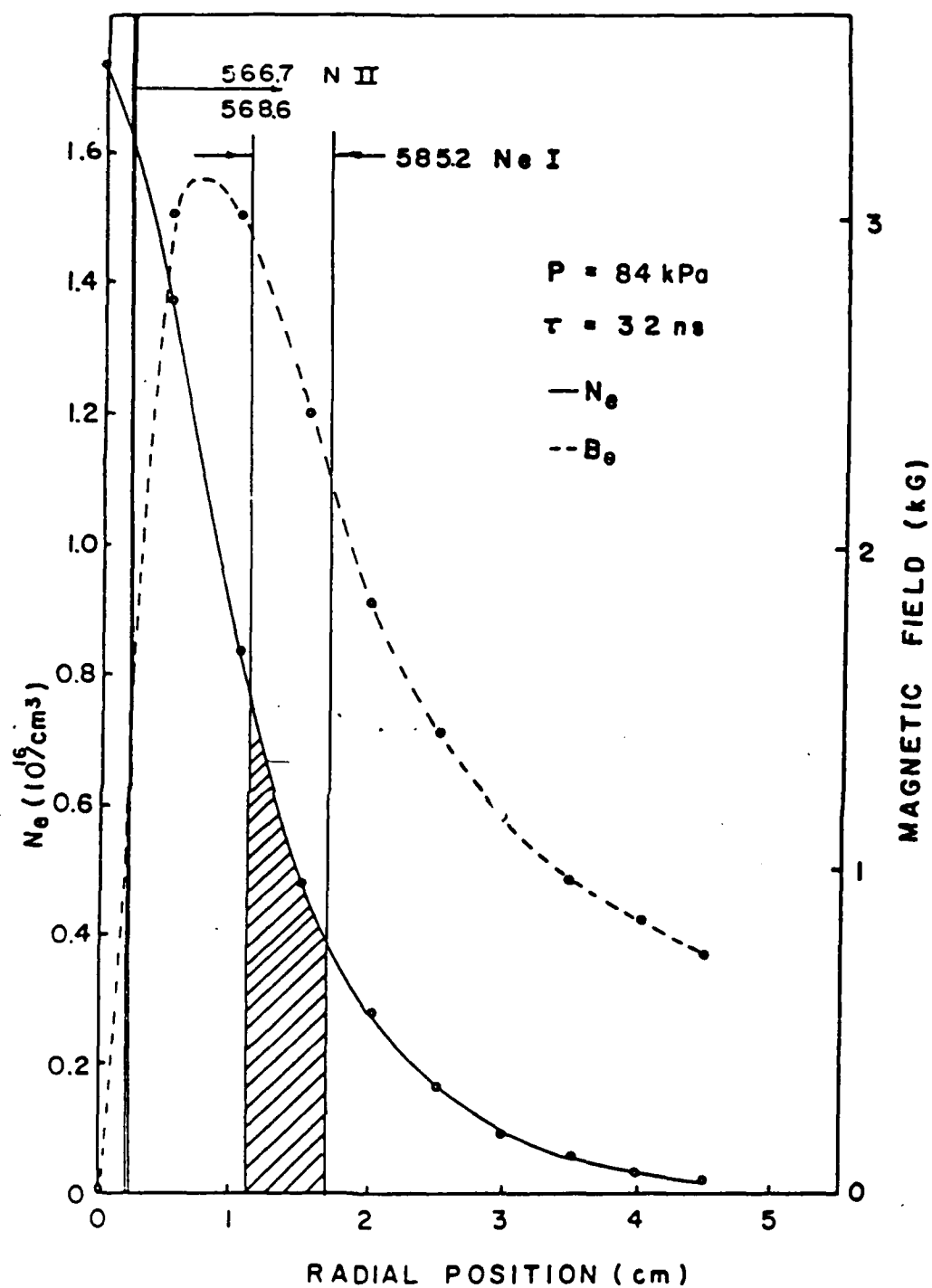
Figure 6. Regions of accessibility to magnetic field measurements on a 20-kA REB using LIF for the 585.2 line of neutral neon (shaded area) and the 566.7 and 568.6-nm lines of ionized atomic nitrogen (to the right of the double verticle lines).
