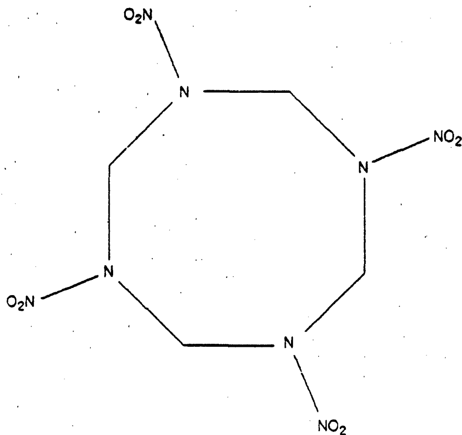
1,3,5,7-Tetranitro-1,3,5,7-tetrazacyclooctane (HMX)
