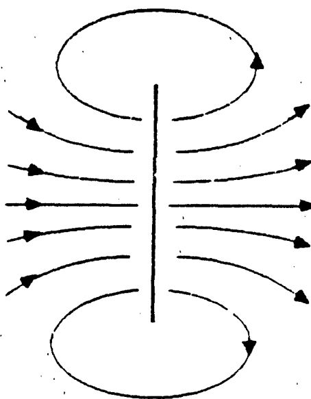
Spiral Coil (Edge View) with Field Lines
