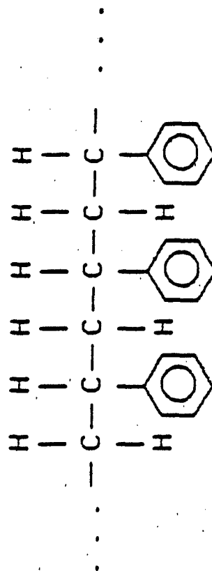
Molecular Structure of Polystyrene
