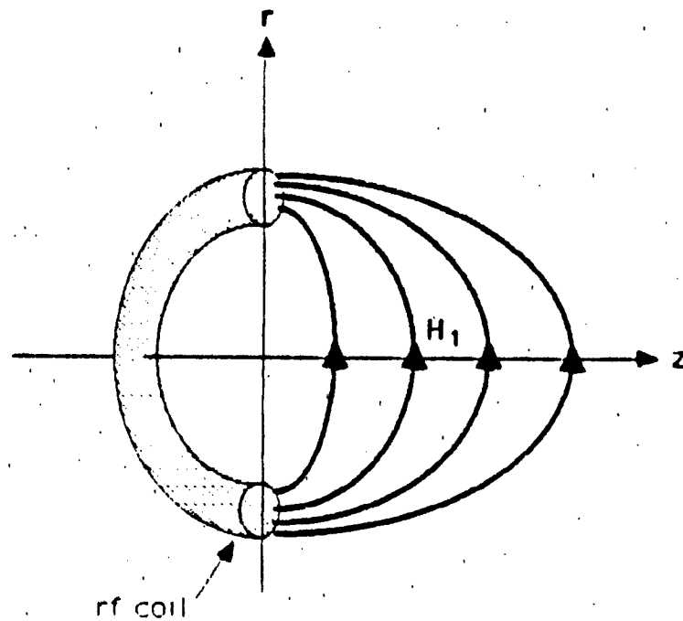
Schematic of Semitoroid RF Coil
