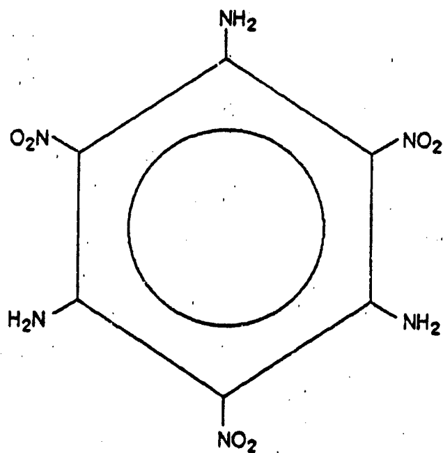
1,3,5-Triamino-2,4,6-trinitrobenzene (TATB)
