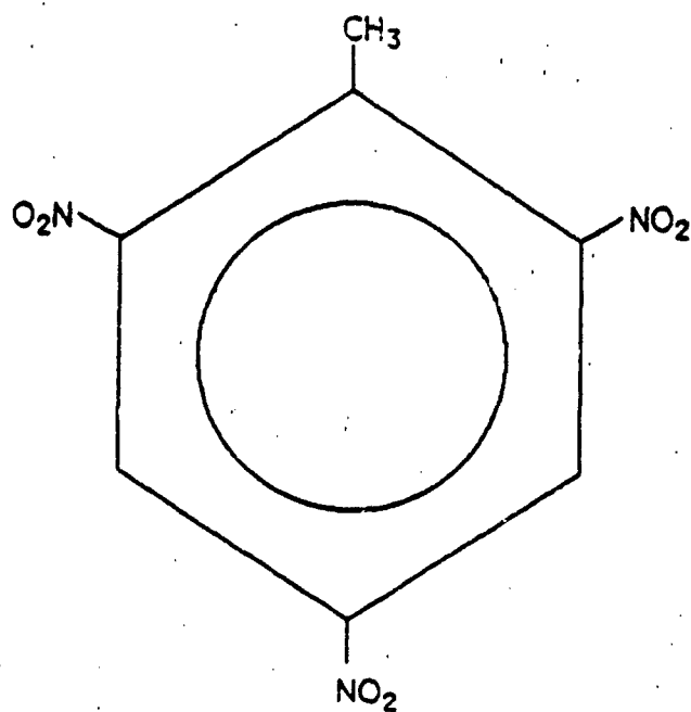
2,4,6-Trinitrotoluene (TNT)
