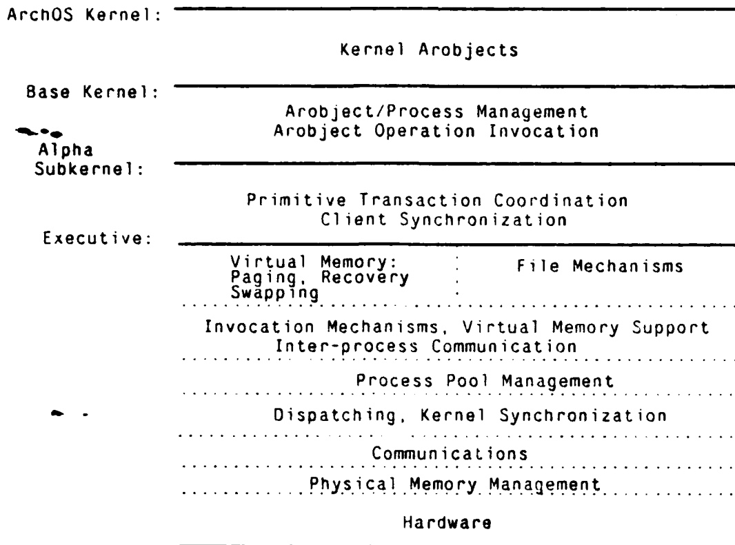
Figure 6-1: Logical Structure of ArchOS Kernel
