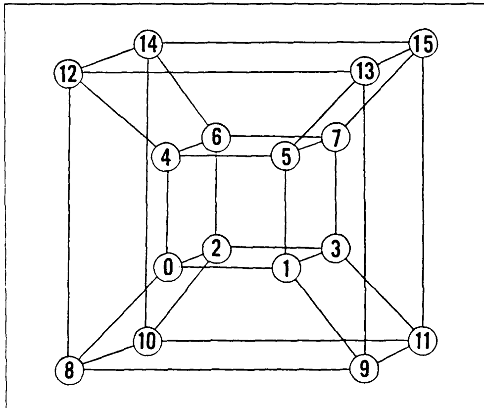
Figure C.2 4-Dimensional Hypercube Topology.
