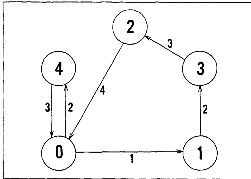
Figure 4.4 Four Equation Train Scheme.
