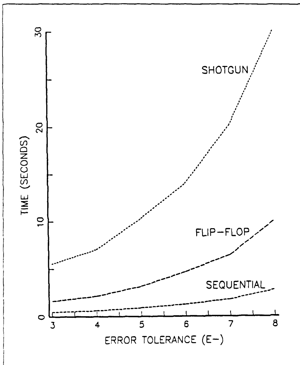
Figure 5.1 Results for the Two Equation System.
