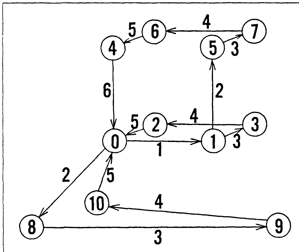
Figure 4.5 Ten Equation Train Scheme.
