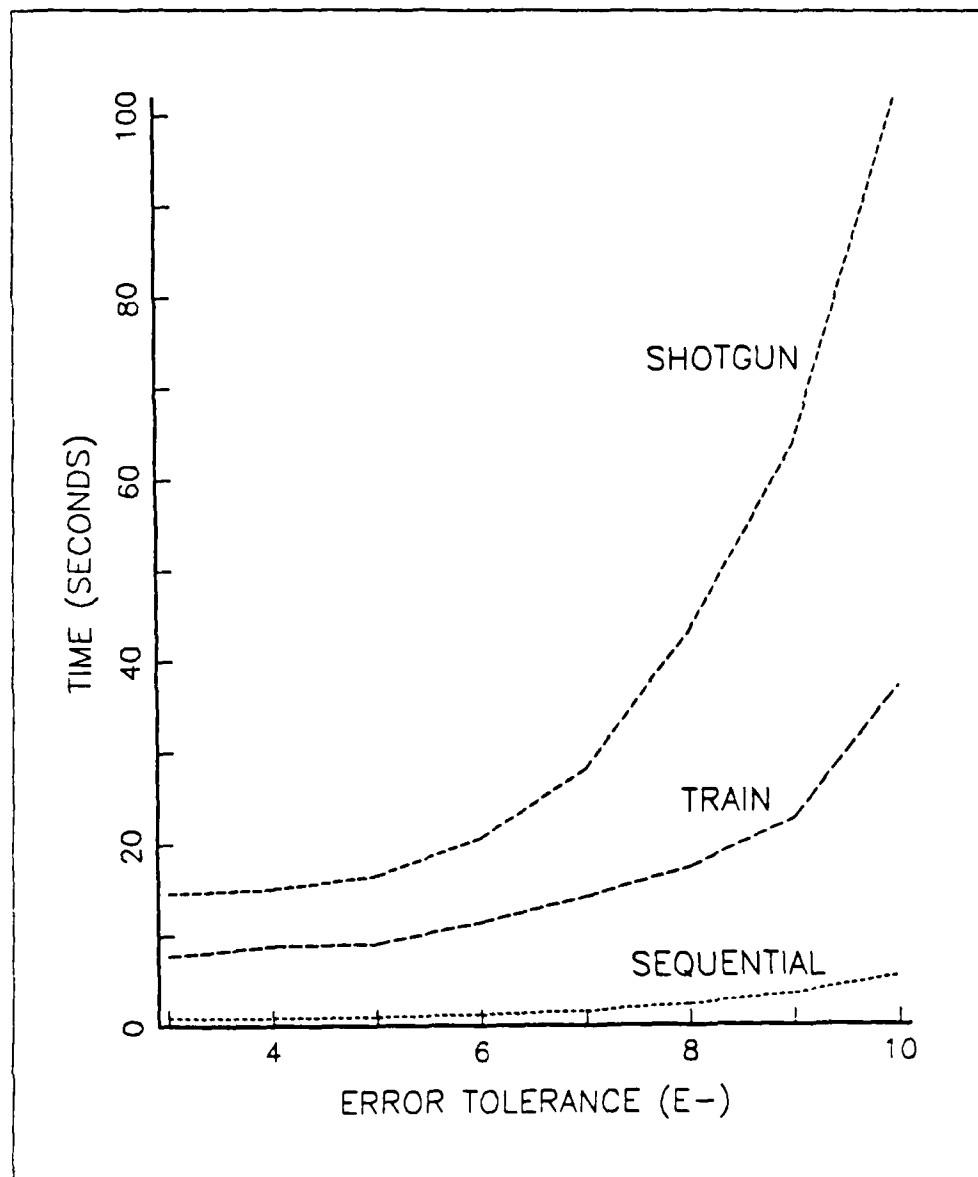
Figure 5.4 Results for the Ten Equation System.
