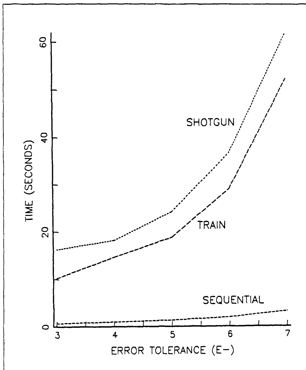
Figure 5.2 Results for the Three Equation System.
