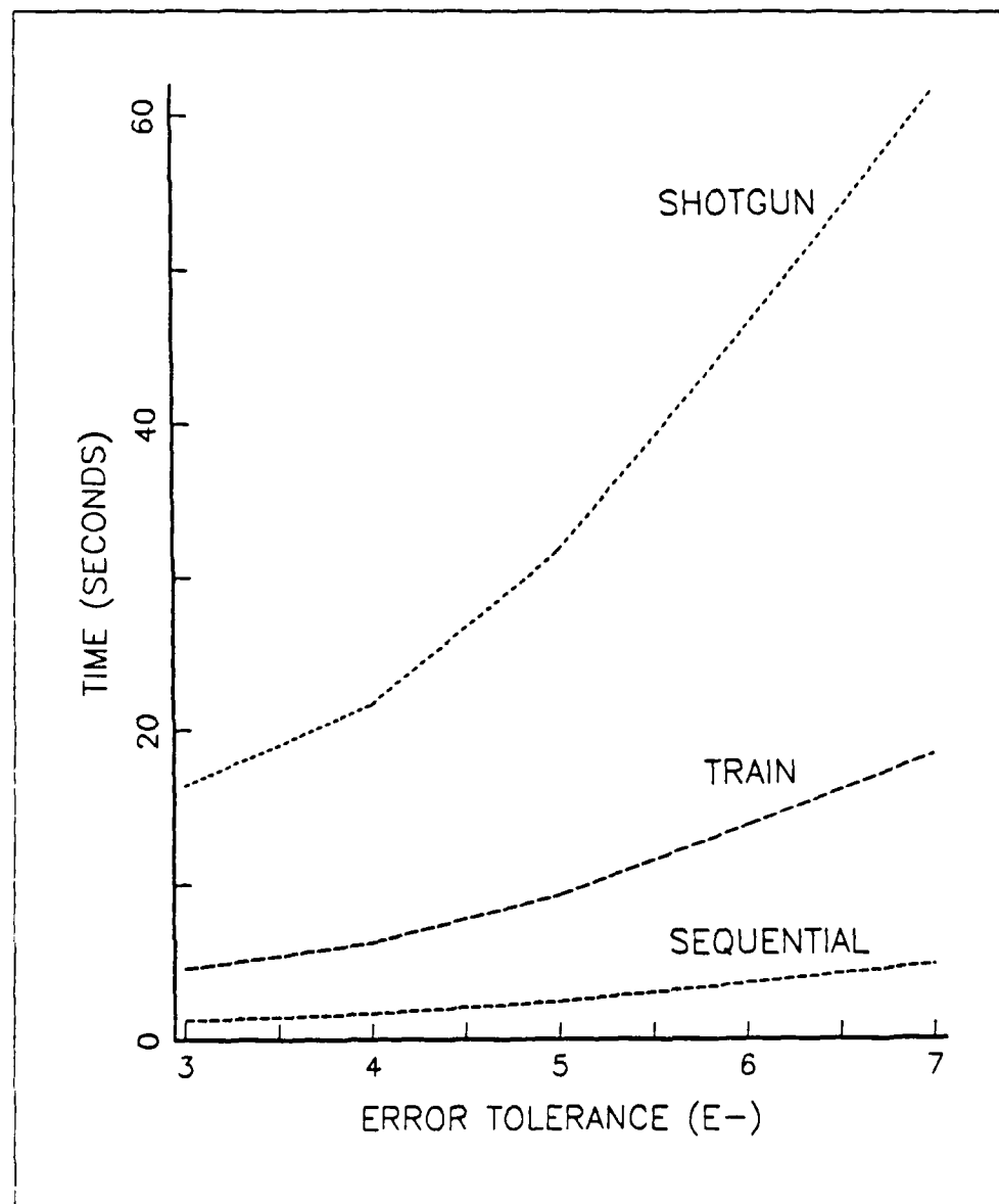
Figure 5.3 Results for the Four Equation System.
