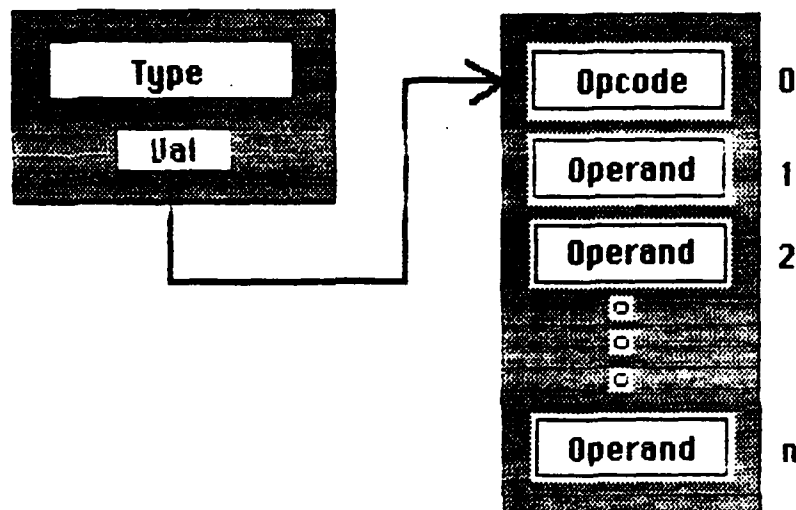
Figure 3.5: Structure of Instruction Value
