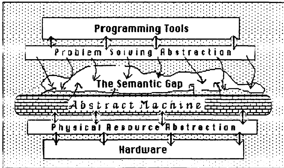
Figure 2.3: Narrowing the Semantic Gap
