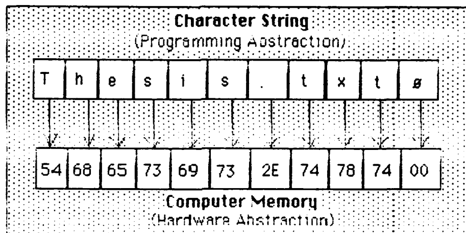
Figure 2.2: Data Type Dependency on Hardware Values
