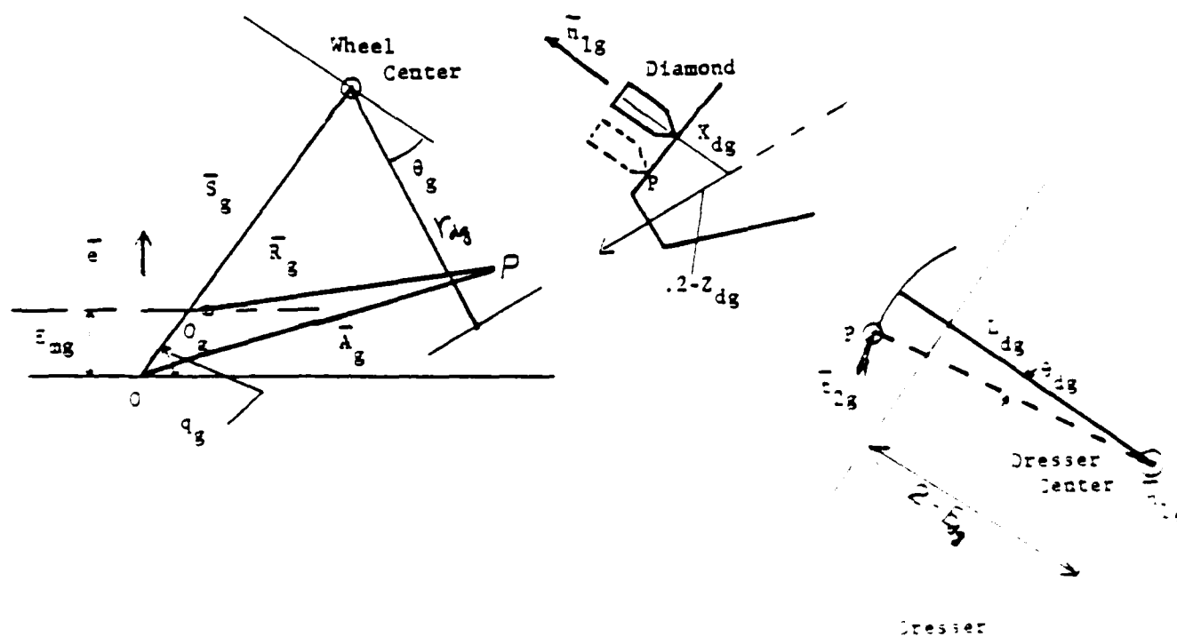
Fig. 2-14. Position Vectors in Machine Plane (Gear
