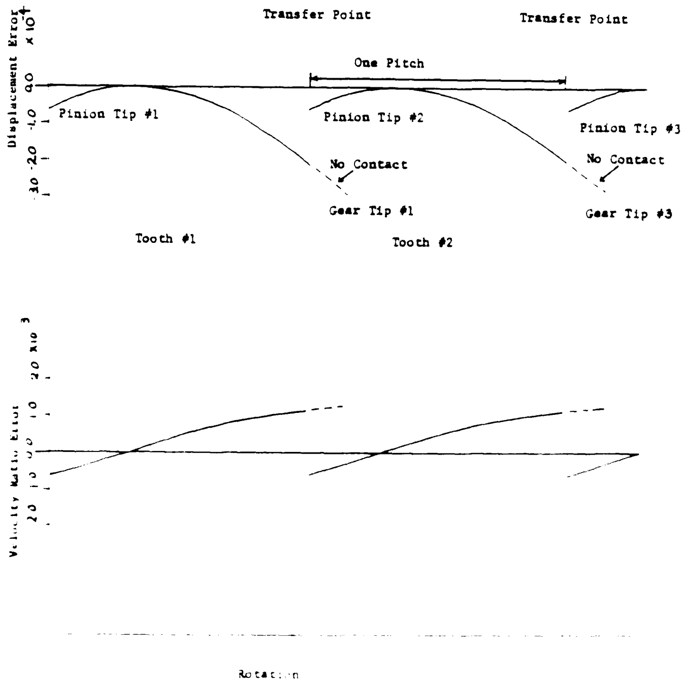
Fig. 1-10. Drive side for a sensitive drive mesh.
