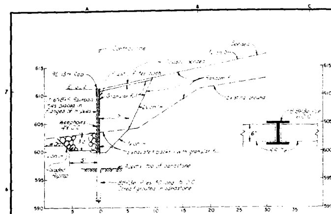
RAILROAD TIE - PILE DETAIL
