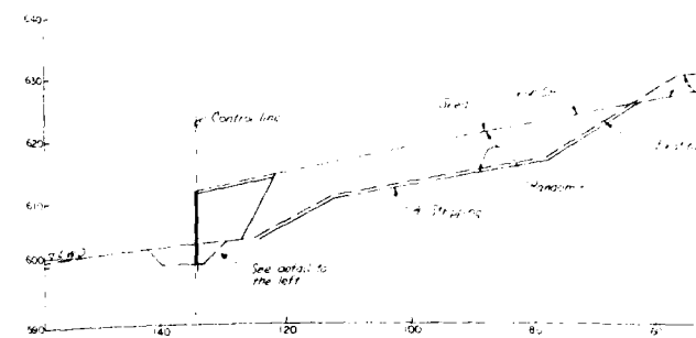
H-PILE AND RAILROAD TIE CROSS SECTION
