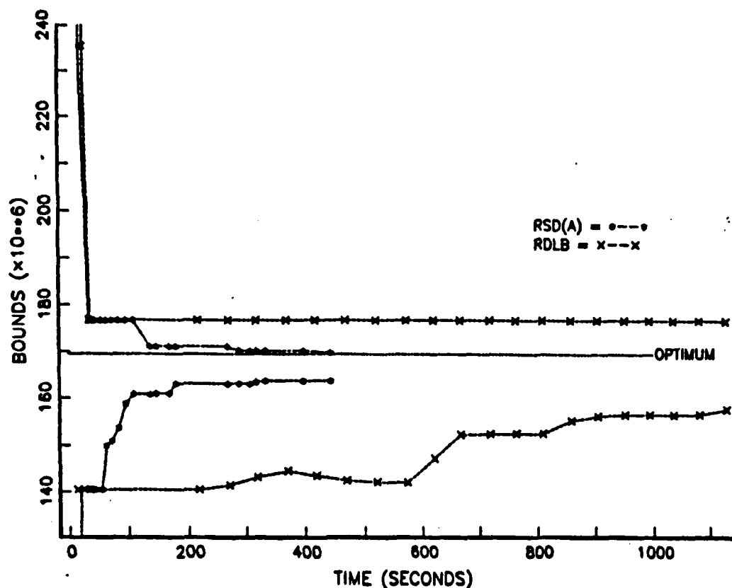
Figure 4.7 Solution Trajectory Comparison (Problem 10H) RSD(A) vs. RDLB
