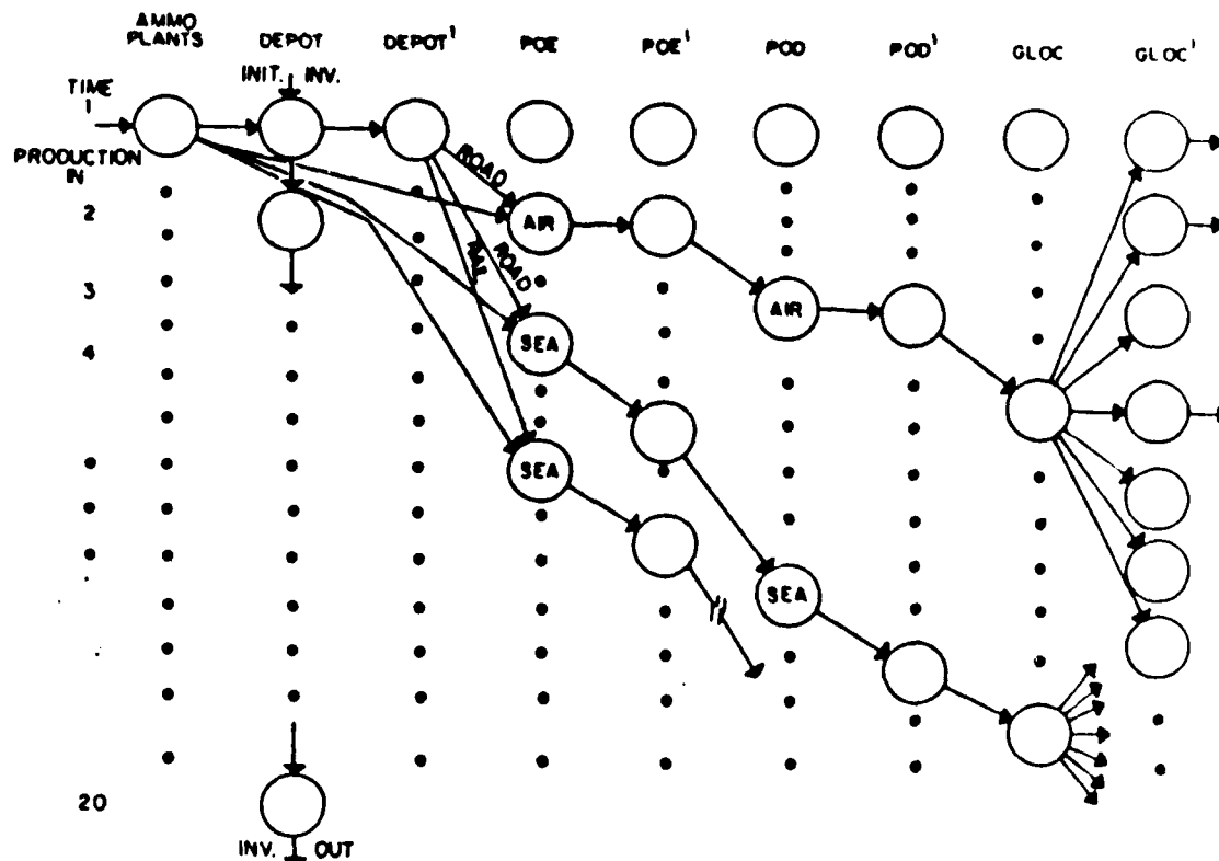
Figure 4.1 Simplified Ammunition Distribution Model
