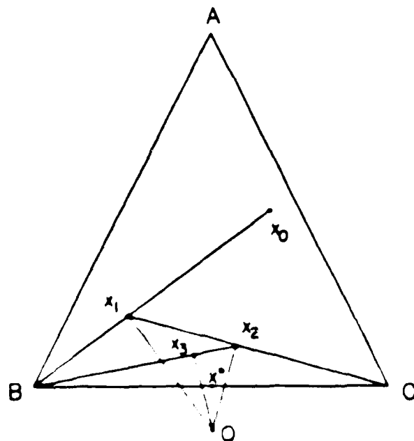
Figure 3.2 Frank-Wolfe Zigzagging Example
