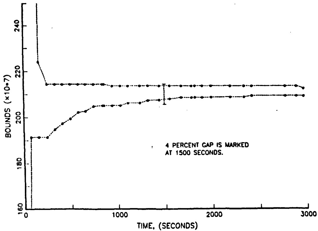
Figure 4.12 Solution Trajectory RSD(A) on 100 Commodities
