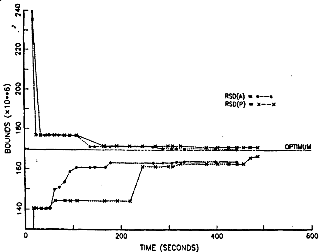
Figure 4.9 Solution Trajectory Comparisons (Problem 10H) RSD(A) vs. RSD(P)
