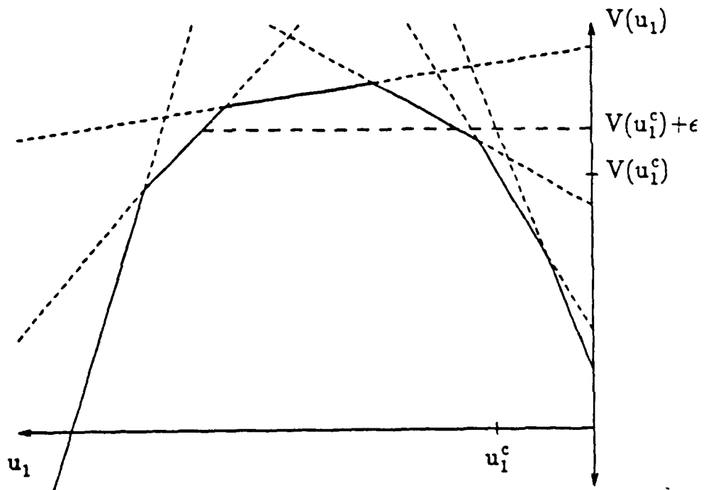
Figure 3.1 Tangential Approximation to Lagrangean Dual Function
