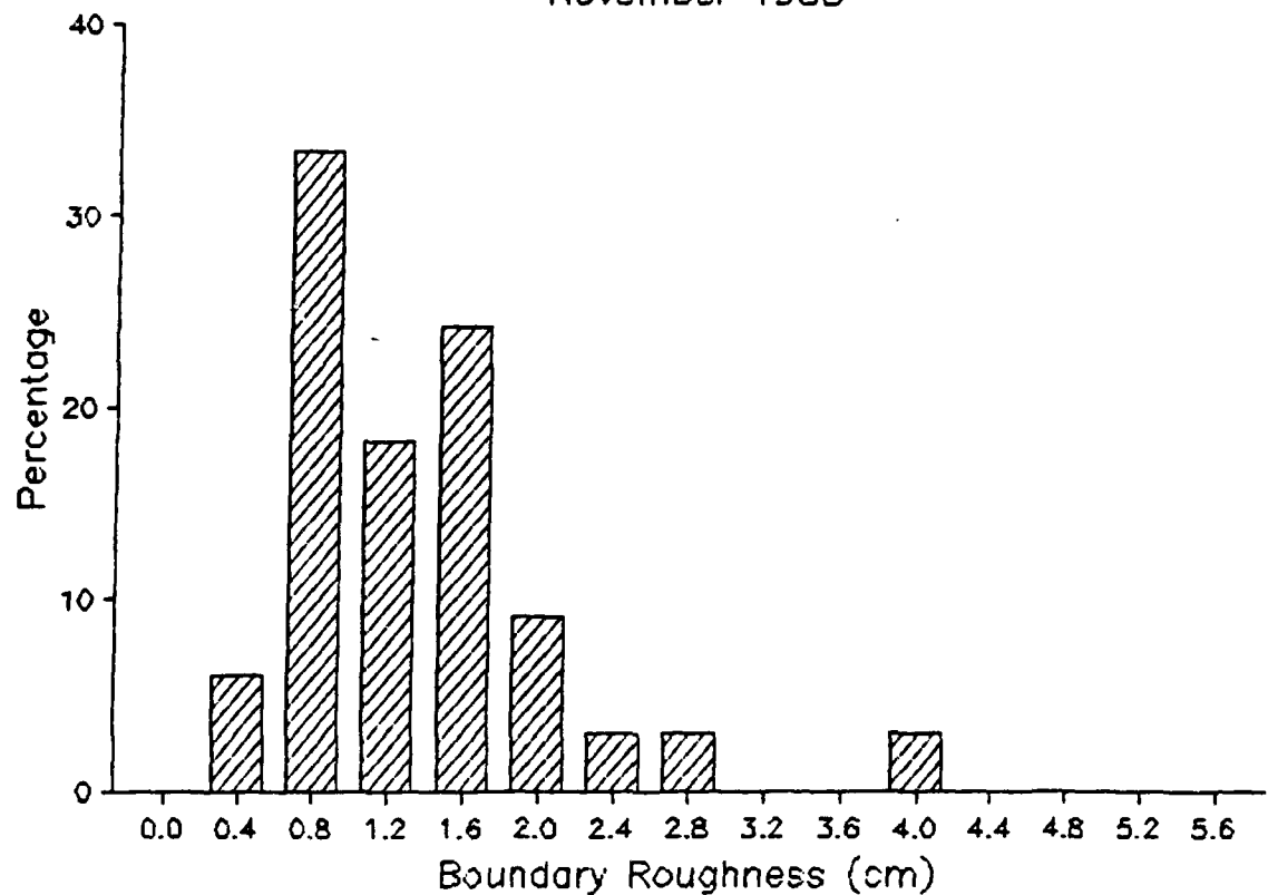
Figure 3.6.3. Histogram of Small-scale Boundary Roughness in the Inner Elliott Bay ZSF
