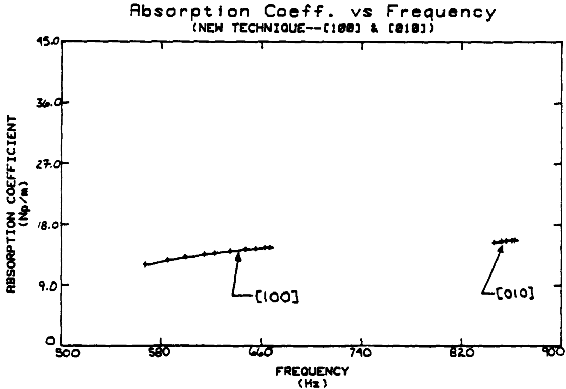
Figure 3.25 a vs f For New Method ([100] and [010] Modes)
