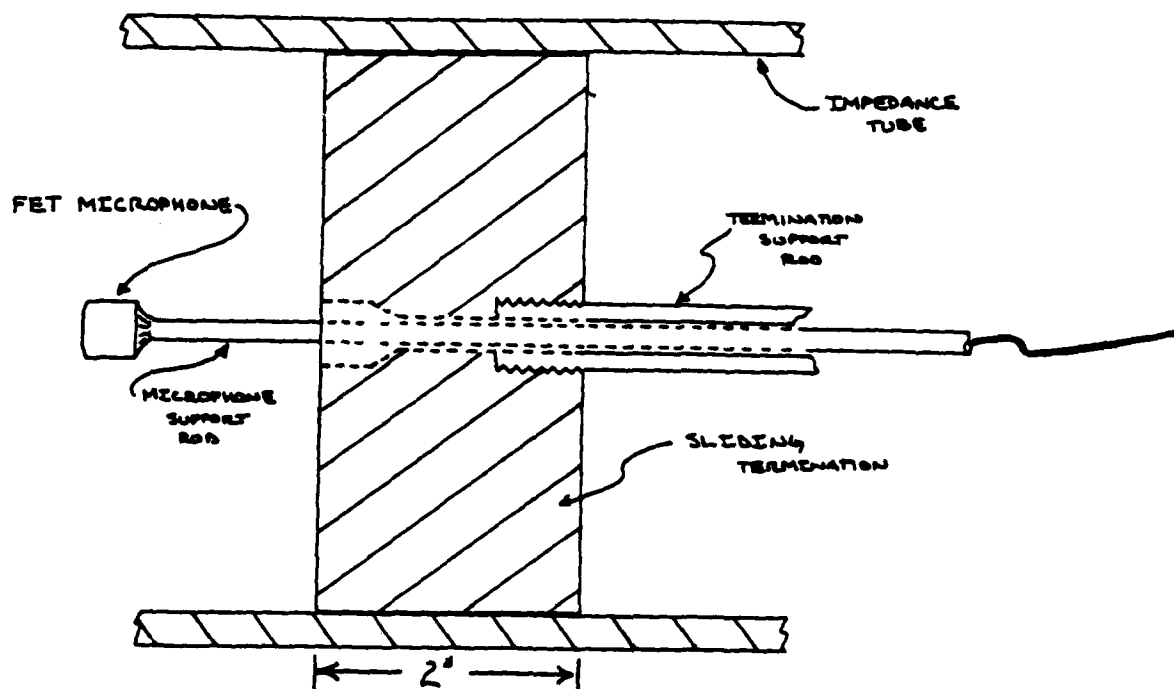
Figure 3.7 The Rigid Sliding Termination (Yaniv's Method)
