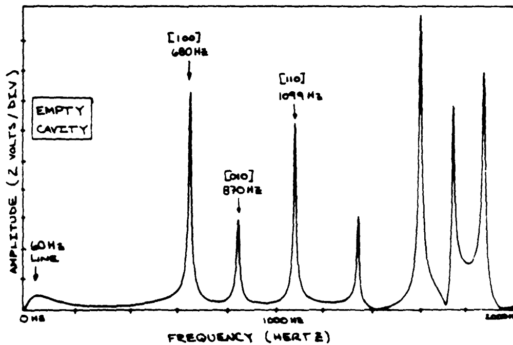
Figure 3.13 Mode Structure of the Empty Cavity
