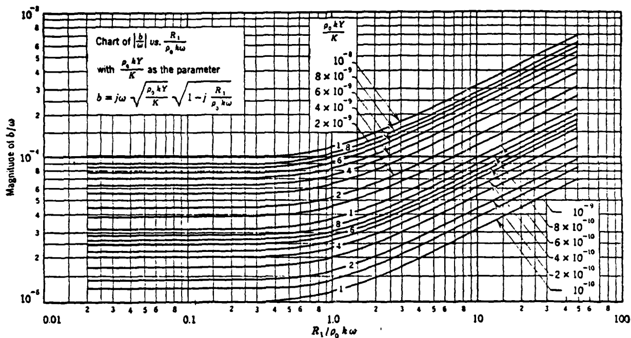
Figure 2.6 Chart for Determining the Magnitude of the Propagation Constant \tilde{b} of Rigid Tiles [Figure 19.3 of Ref. 4, p. 843]
