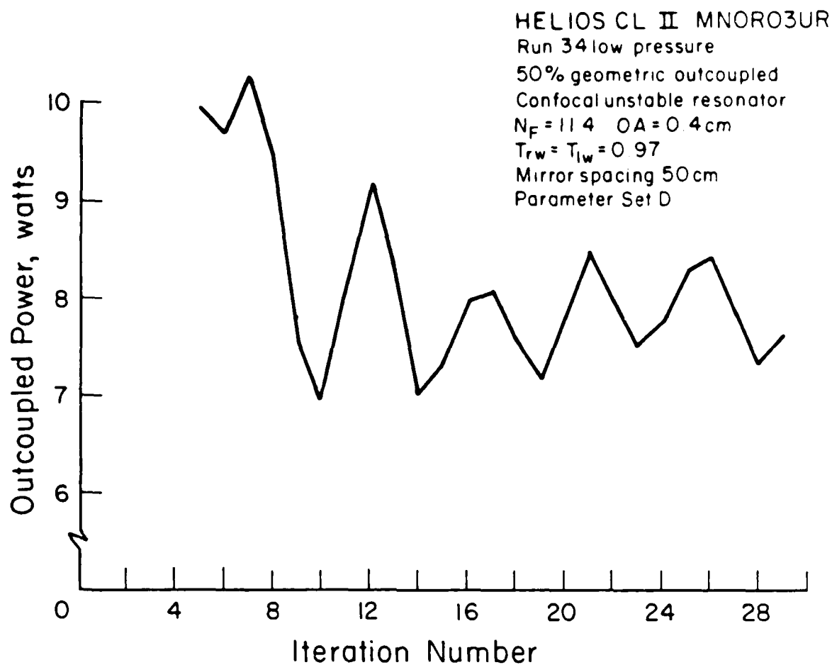
Figure 39 MNORO3UR outcoupled power 8 , P_{out} , for individual lines vs. iteration number for a 50% geometric outcoupled, confocal, unstable strip resonator with a large mirror diameter of 0.8 cm for the Helios CL II laser for Run 34 at 5.4 Torr.
