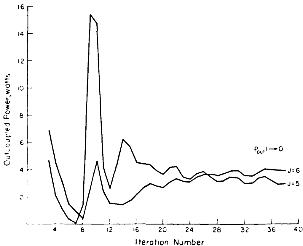
Figure 34 MNOR03UR outcoupled power 8 , P_{out} , for individual lines vs. iteration number for a 50% geometric outcoupled, confocal, unstable strip resonator with a large mirror diameter of 1.0 cm for the Helios CL II laser for Run 34 at 5.4 Torr.
