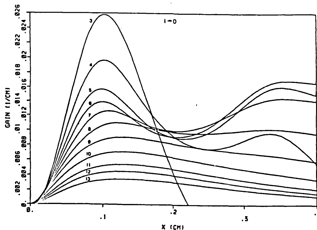
Figure 13 MNOR03UR gains at iteration 23 for a 50% geometric out-coupled, confocal unstable strip resonator with a large mirror diameter of 4 mm for the Helios CL II for the low pressure Run 34 flow rates.
