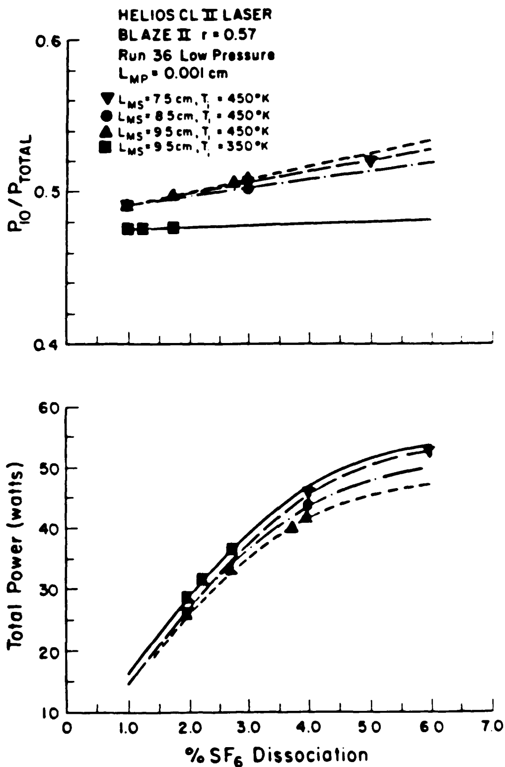
Figure 9 Variation of total power and fraction of power in the 1-0 vibrational band 1 as a function of percent \text{SF}_6 dissociation from the BLAZE II model of the CL II laser, L_{MP} is the mixing length of the primary stream, L_{MS} is the mixing length of the secondary stream.
