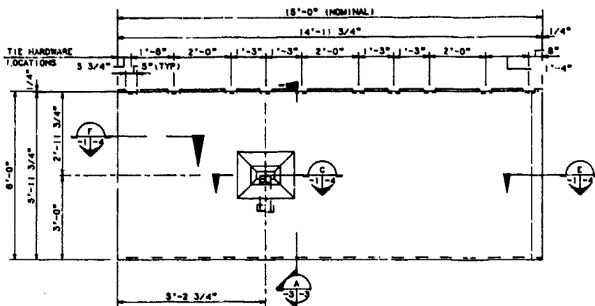
ELEVATION - PRECAST PANEL 'P-7' SCALE: 1/2"=1'-0"
