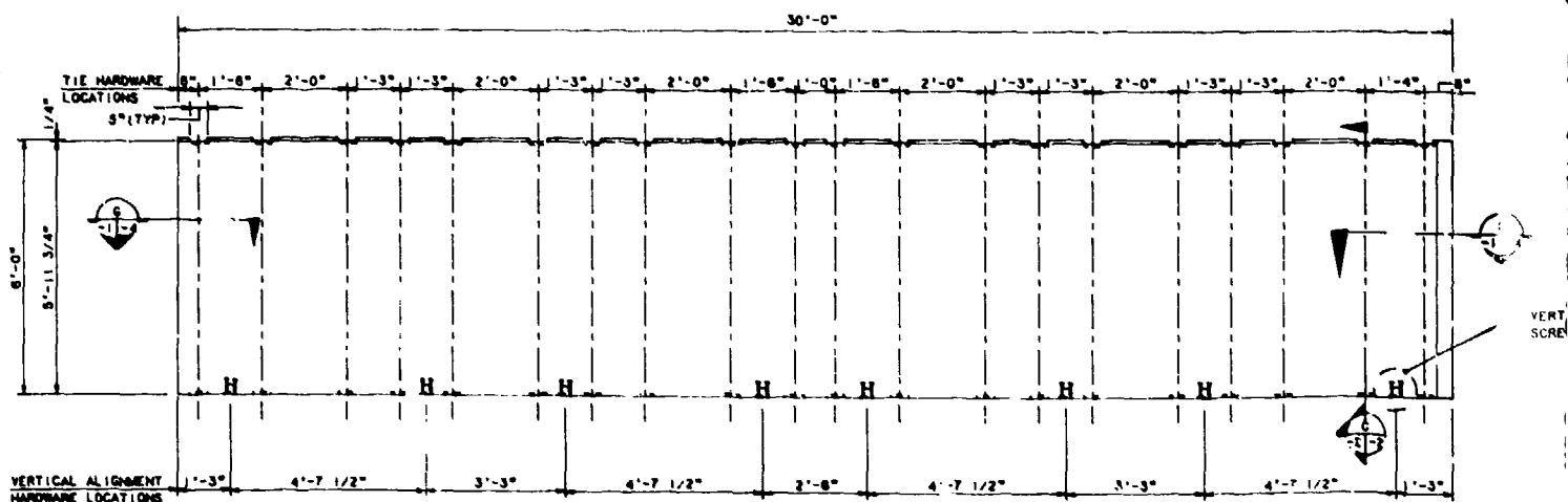
ELEVATION - PRECAST PANEL 'P-1' SCALE: 1/2"=1'-0"
