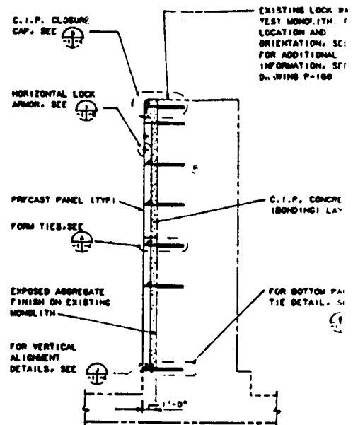
SECTION - LOCK SURFACE REHABILITATION SCALE: 1/4" = 1'-0"
