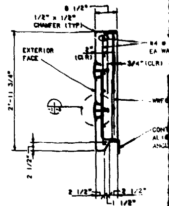
SECTION - PRECAST PANEL 'P-5' & 'P-4' SCALE: 1/2"=1'-0"
