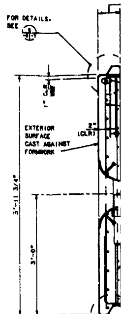
SECTION - PRECAST PANEL 'P-8' SCALE: 1/2"=1'-0"
