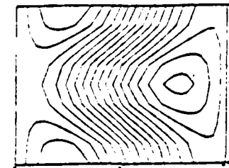
Figure 1 : Streamlines of the steady finite amplitude two-dimensional traveling wave for plane Poiseuille flow at Re = 6000 , plotted in the rest frame of the wave (from ref. [2]).
