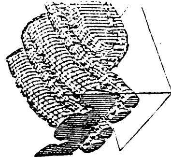
Figure 4 : A plot of the region of low vorticity in the secondary instability of mixing layer flow (from ref. [6]). The rollers connecting the large rollers are regions of significant streamwise vorticity in which \omega is nearly aligned with y .
