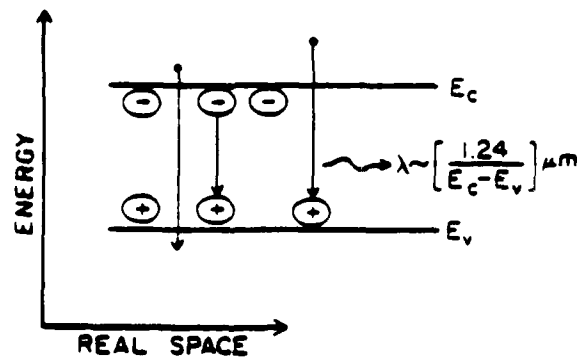
(b) Bulk Al_xGa_{1-x}As Optical Transitions
