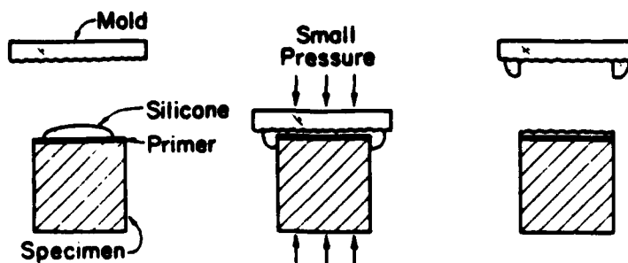
Fig. 2 The crossed-line specimen grating was replicated at 250°F.
