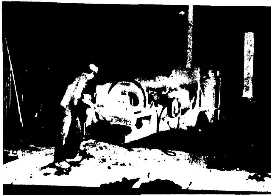
Figure 15. Porta-Patcher® Used to Recycle Asphalt Concrete Pavement During Reconstruction of Test Sections.
