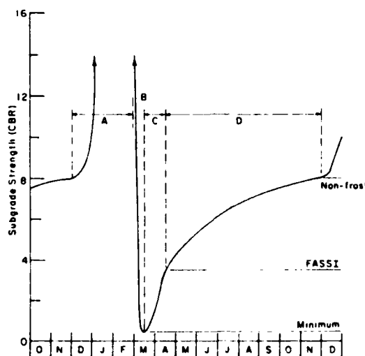
Figure 31. Change in CBR of an F4 Subgrade Soil that Freezes in Winter.
