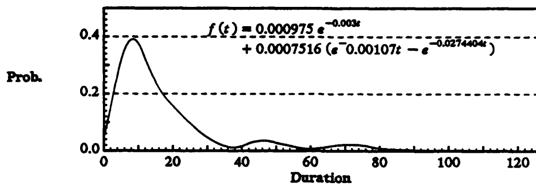
Holding time density to DASD
