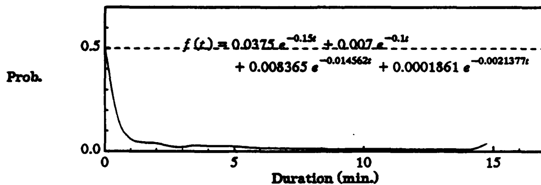
Waiting time density of DASD
