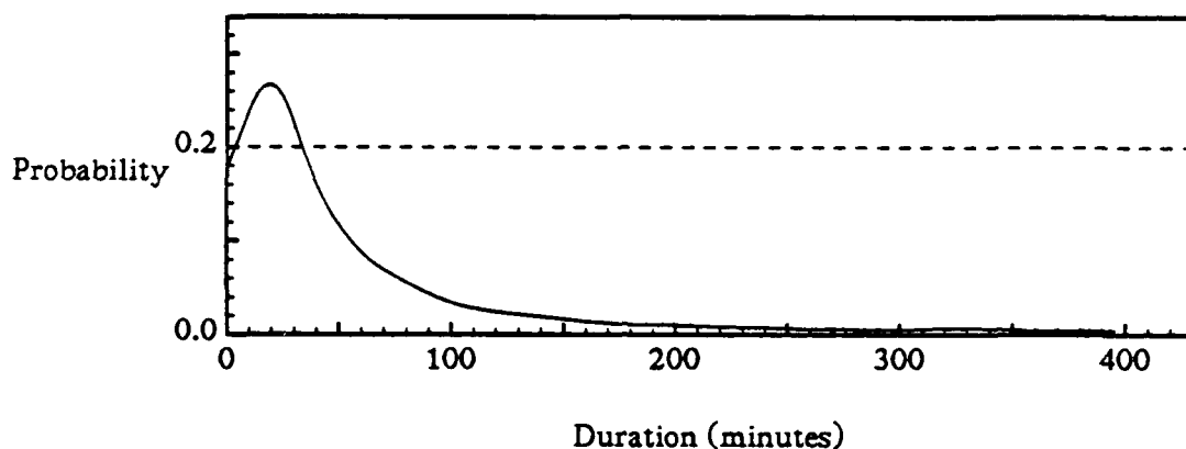
Figure 4.5. Time to error density
