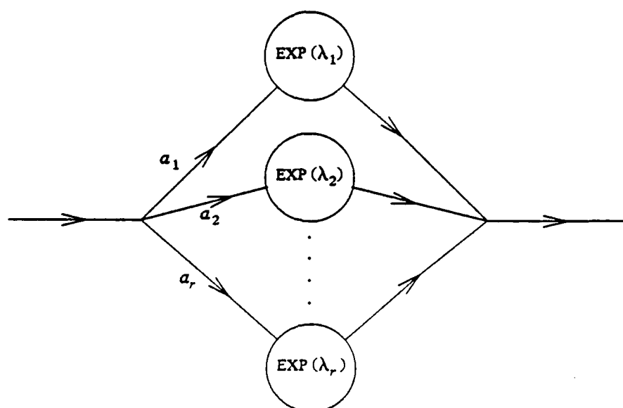
(a). Hyperexponential distribution as a set of parallel exponential stages
