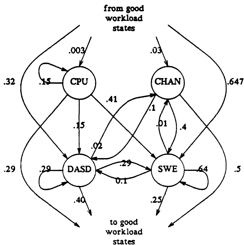
Figure 2.5. State-transition diagram for multiple errors (MULT)
