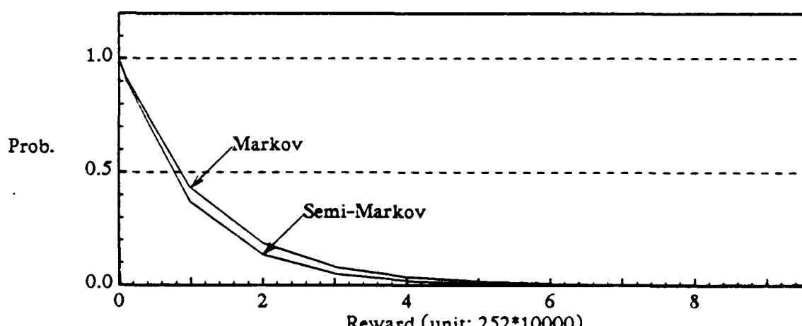
Figure 5.5. Distribution of accumulated reward until system failure
