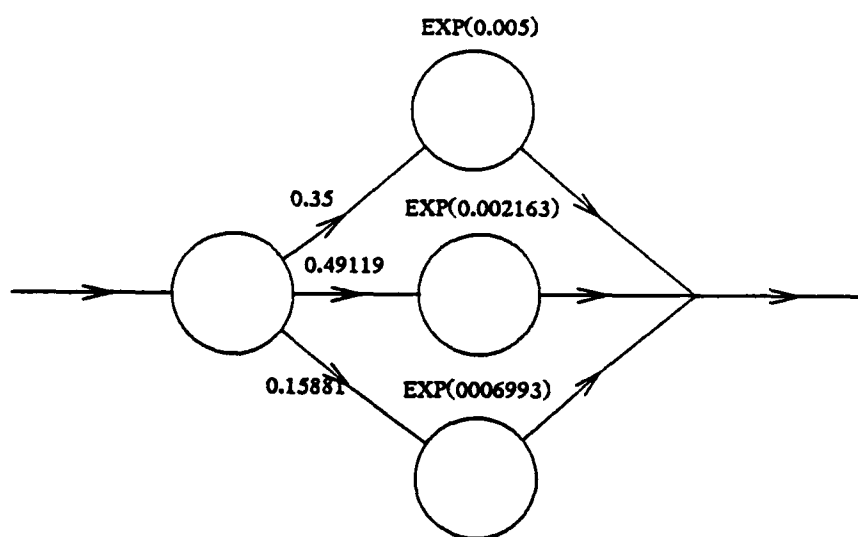
(b). W_3 state
