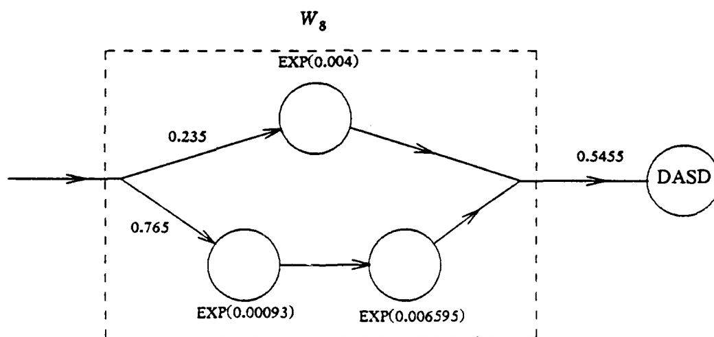
(b). Markov
