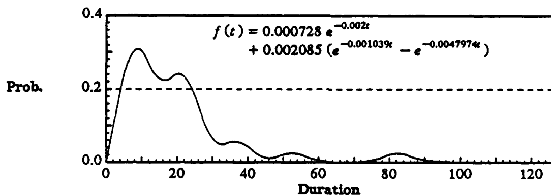
Holding time density to SWE
