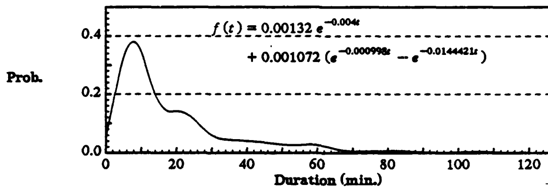
Holding time density to the others
