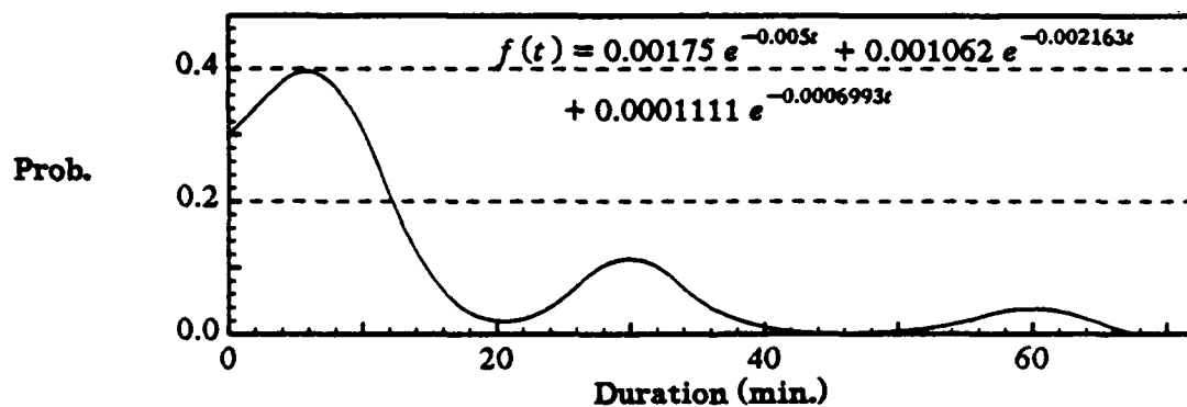
Waiting time density for W_3
