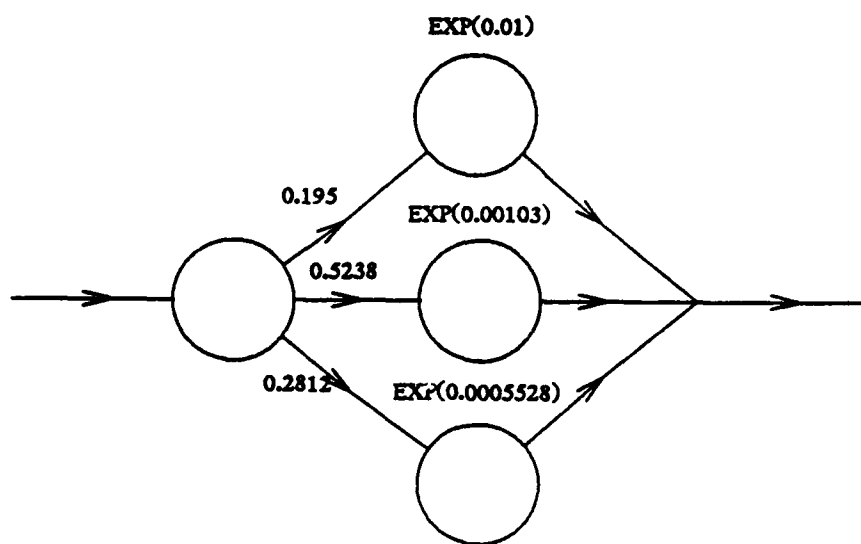
(a). W_1 state
