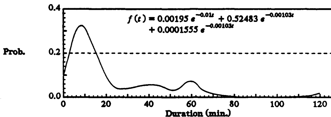
Waiting time density of W_1
