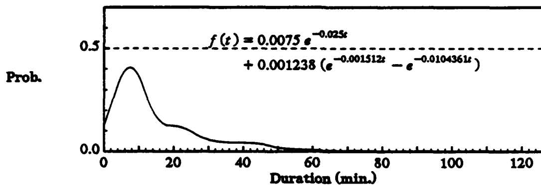
Holding time density to MULT
