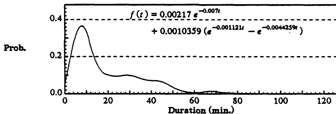
Holding time density to SWE
