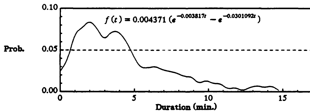
Waiting time density of MULT
