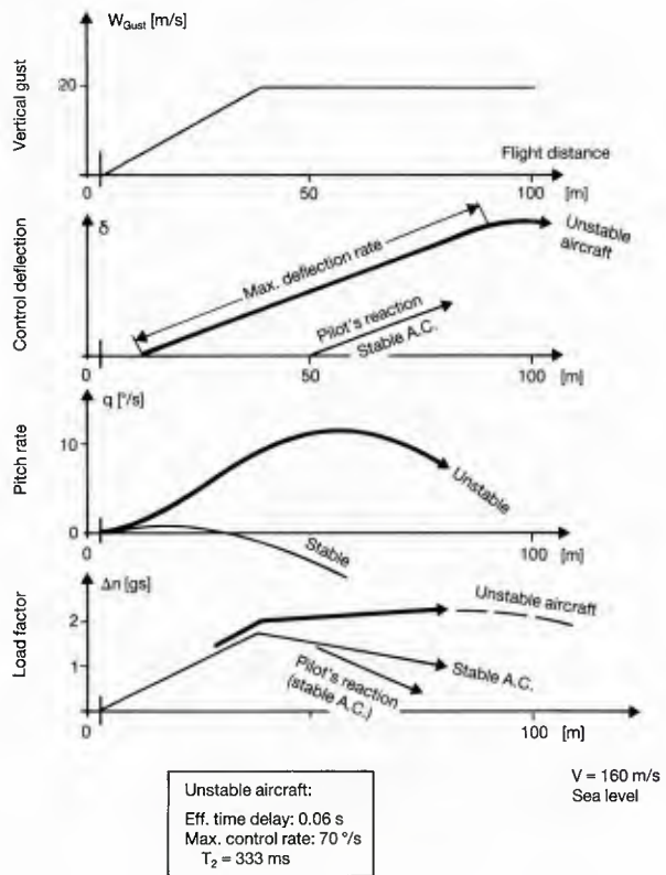
Fig.17 Effect of too Large Instability (Pitch Up) on Gust Response (Sample Aircraft)
