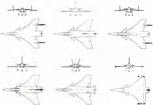
FIG. 6 - EXAMPLE OF DELTA-CANARD CONFIGURATIONS STUDIED
