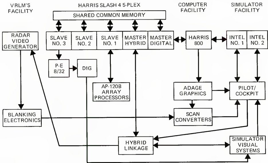
FIGURE 36. TYPICAL FACILITY FUNCTIONAL FLOW SCHEMATIC
