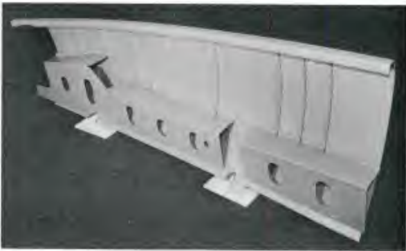
FIG. 13 - RAFALE FRONT FUSELAGE CARBON FIBER ELEMENT
