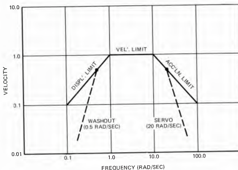
FIGURE 25. MOTION PERFORMANCE DIAGRAM
