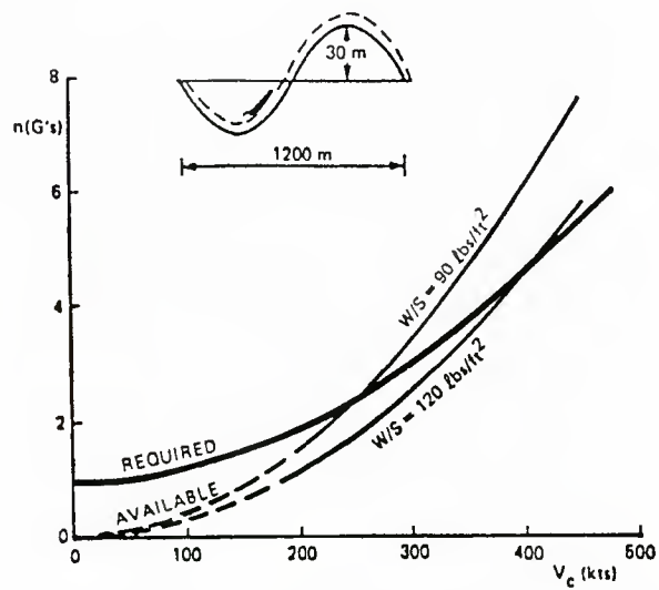
FIG.6: MANOEUVRABILITY REQUIREMENTS
