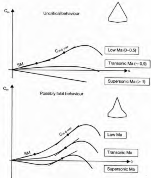
Fig. 28 Pitch Behaviour of Unstable Aircraft (Zero Controls) for Different Mach-Number Ranges
