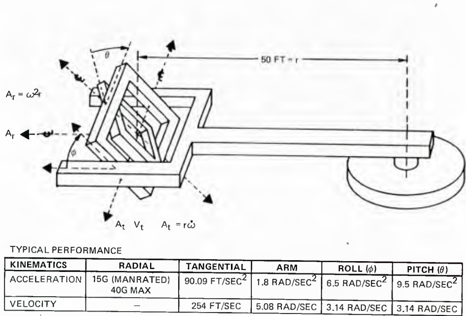
FIGURE 12. CENTRIFUGE MOTION SYSTEM
