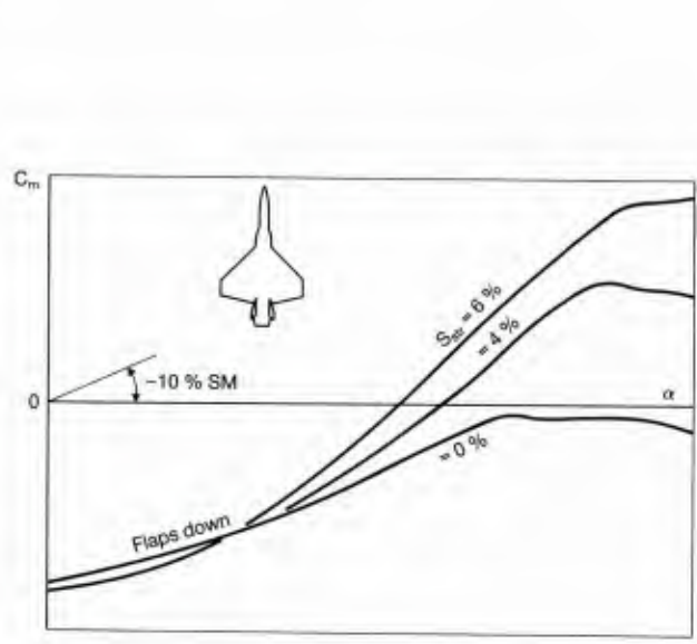
Fig.19 Effect of Wing Strakes on Pitch Behaviour
