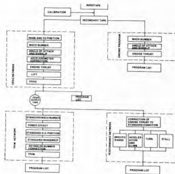
Fig. 7 - Performance Data Analysis Software Network
