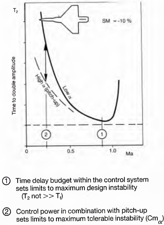
Fig.10 Variation of "Time to Double Amplitude" Versus Mach-Number
