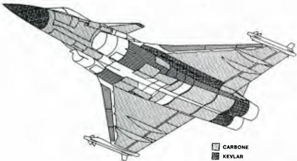
FIG. 14 - NEW MATERIALS IN RAFALE (BOTTOM VIEW)
