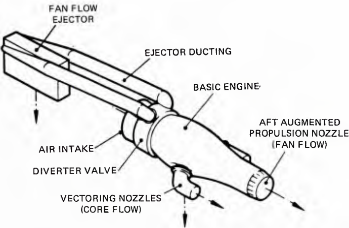
Fig. 22 Separate flow ejector
