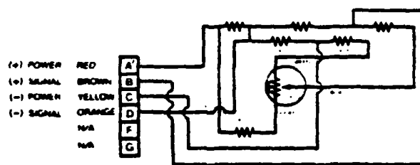
B CIRCUIT
