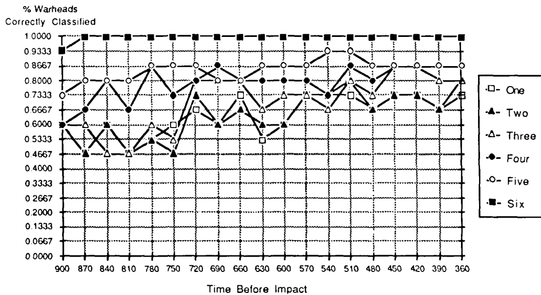
Figure 5.5 Radar Sensitivity
