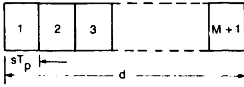
Fig. 1 — Idealized representation of the spot as M + 1 range resolution cells
