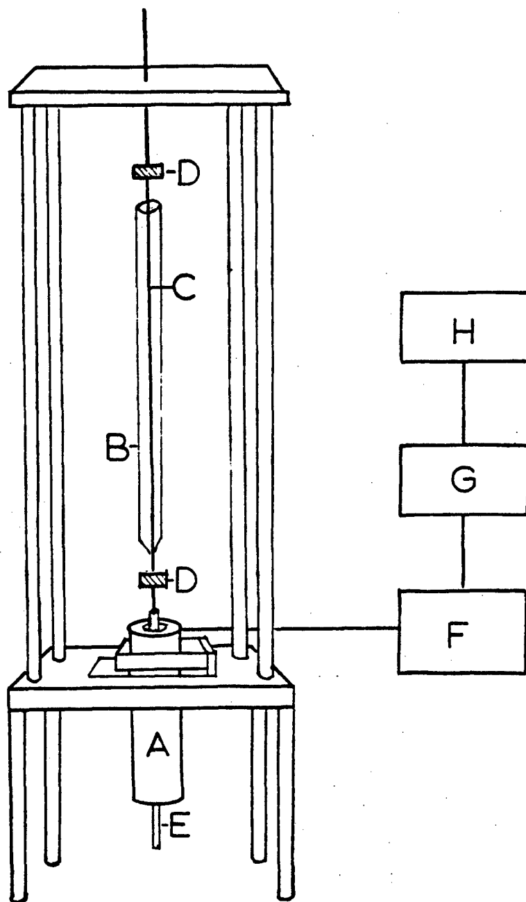
Figure 4 Experimental design for axial displacement measurements during drying.
