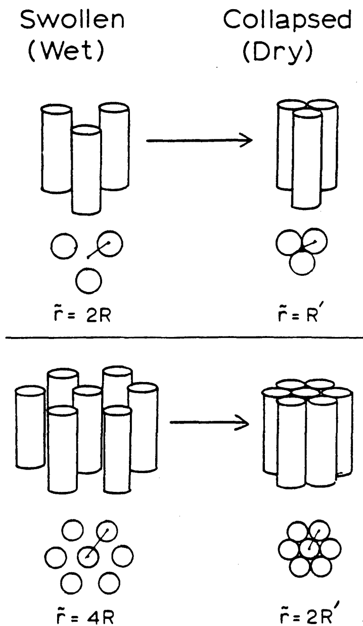
Figure 20. Representation of a PBT fiber composed of 3 and 7 fibrils in the wet and dry state
