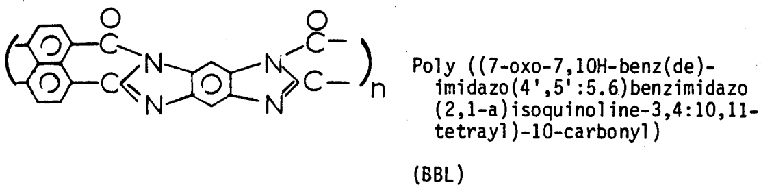
Figure 2. Rod-like aromatic polymers
