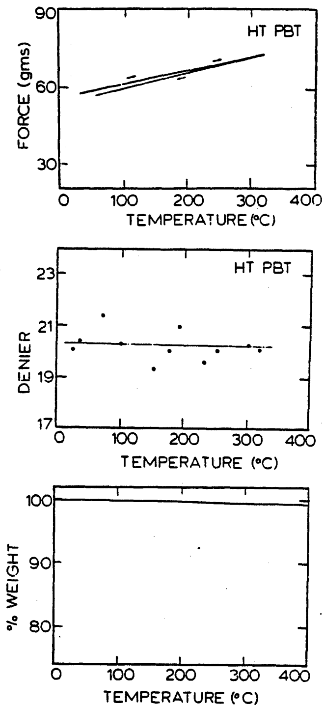
Figure 49 (A) Force-Temperature Profile (B) Denier-Temperature Profile (C) Thermal Gravimetric Profile for heat treated PBT fiber.
