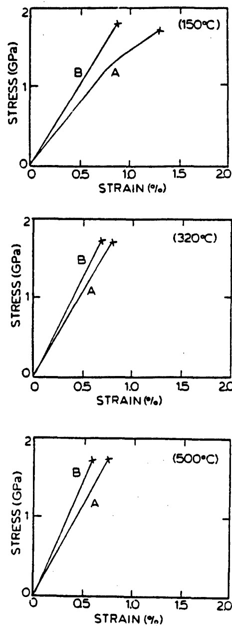
Figure 33 Typical stress-strain curves for PBT fibers dried at 150°C, 320°C, and 500°C at:
