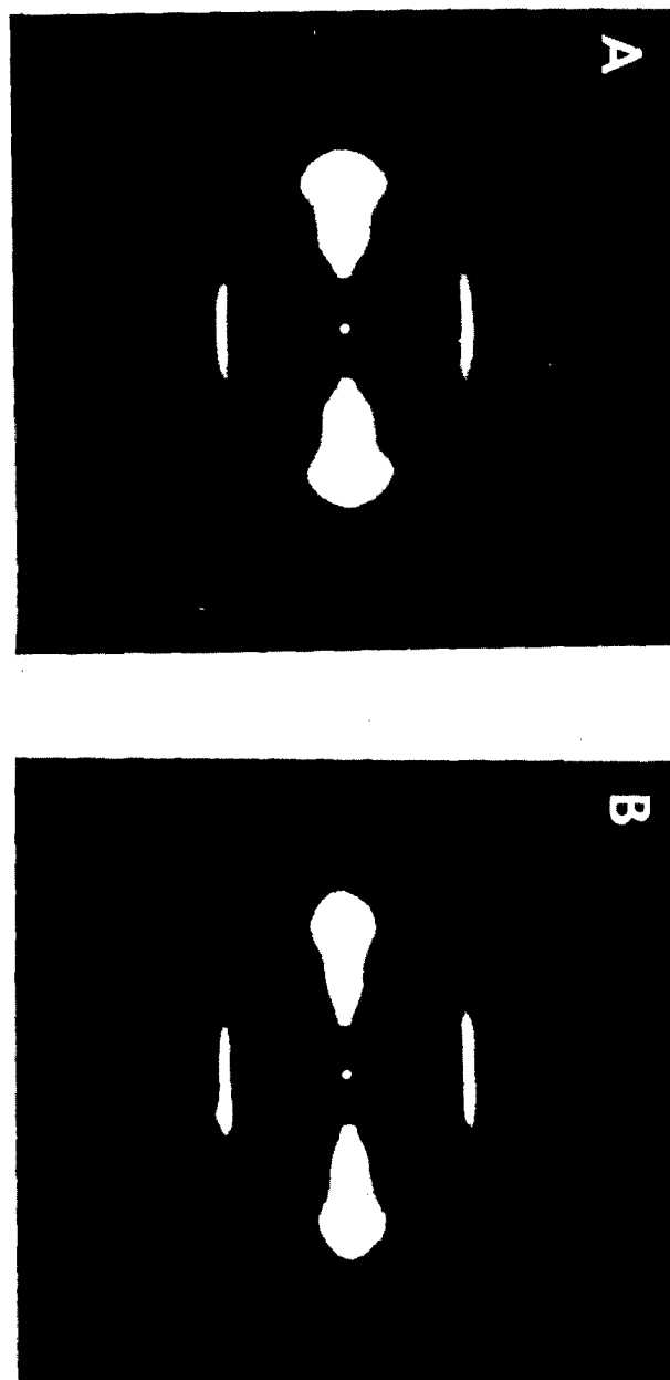
Figure 26 WAXD patterns for PBT Fiber I (A) Non-tension dried (B) Tension dried (300 MPa)
