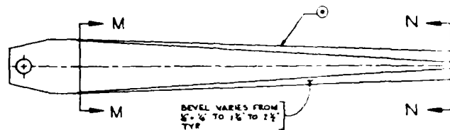
DETAIL A1 - SHANK (CASTING OPTION) SEE DETAIL A FOR DIMENSIONS
