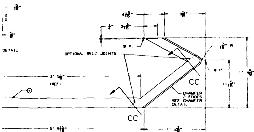
DETAIL C
