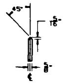
CHAMFER DETAIL
