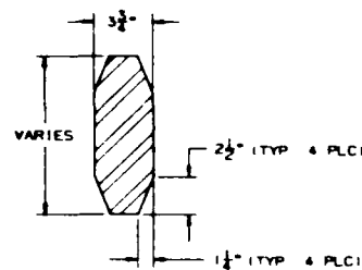
SECTION N-N
