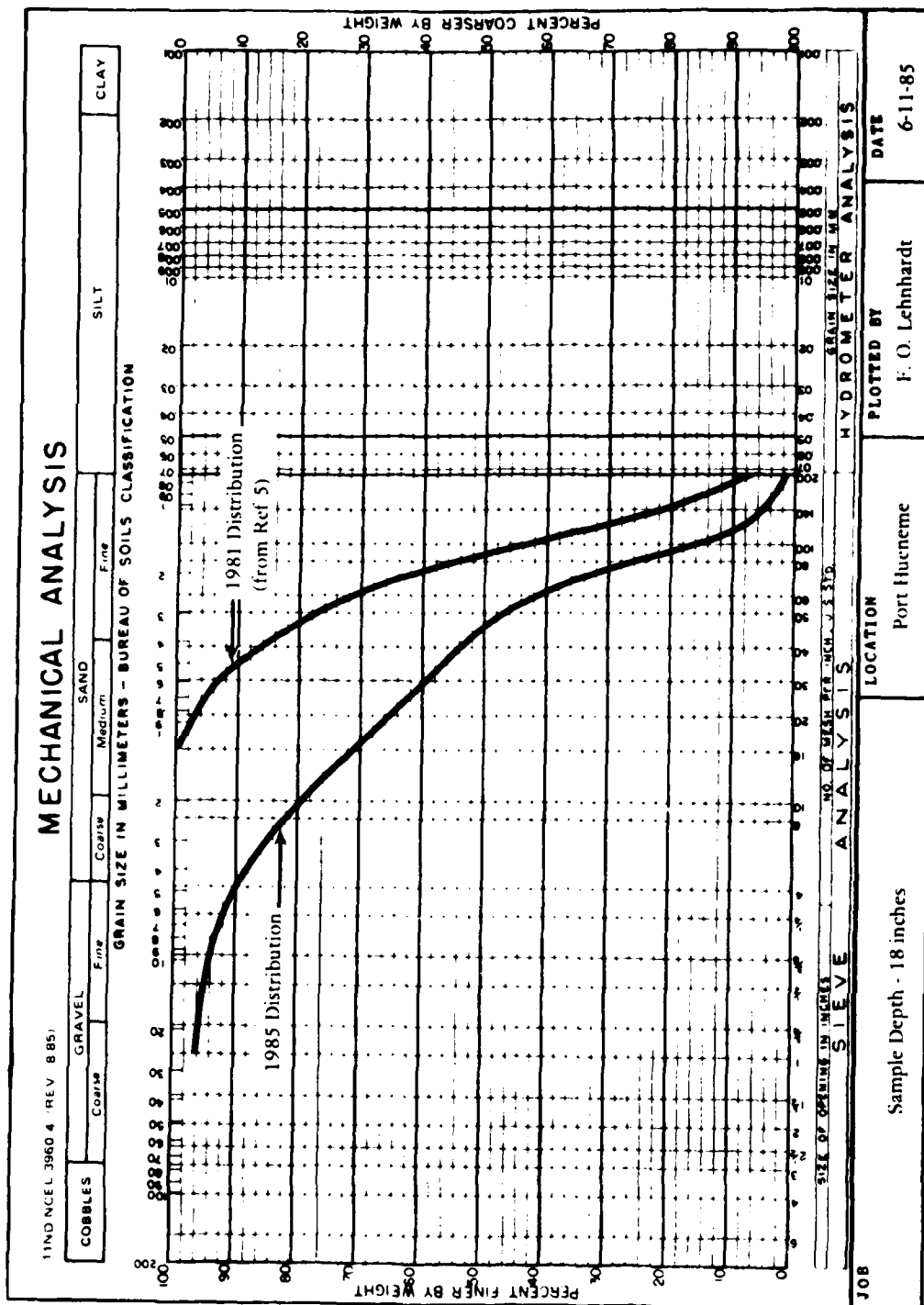
Figure 7. Grain size distribution for Port Hueneme sand, west jetty.
