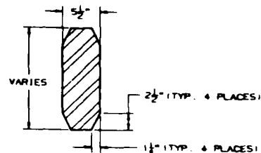
SECTION M-M (SEE NOTE 1)
