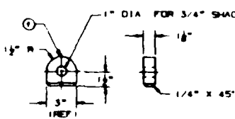
DETAIL F - PAD EYE
