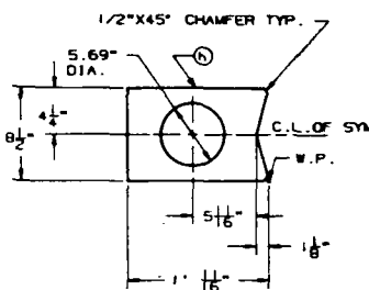
DETAIL H
