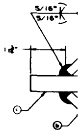
SECTION E
