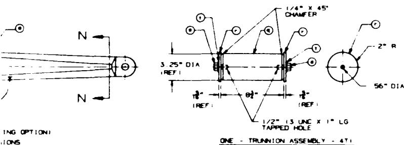
ONE - TRUNNION ASSEMBLY - 471
