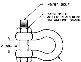
DETAIL B - SHACKLE
