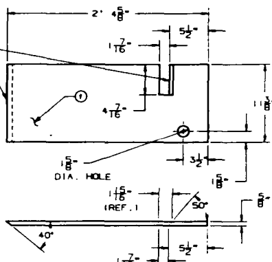
DETAIL F
