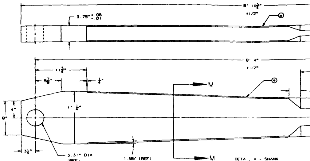
DETAIL A - SHANK
