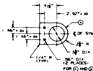
DETAIL K - RETAINING RING
