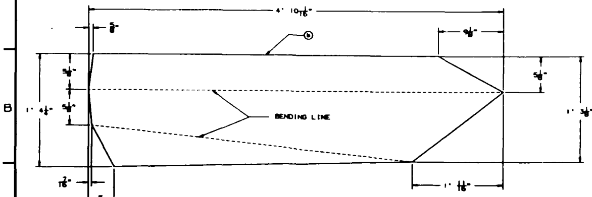
DETAIL B (DEVELOPMENT DETAIL)
