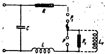
Fig. 2. Diagram of a stable loop with two sparks. The capacitance C is charged through a shunting resistance R_1 or a self-inductance L_1 up to breakdown of the stable regulated gap P_1 . After the breakdown, the voltage is concentrated on the larger resistance R_1 (or L_1 ), which causes breakdown of the gap P under investigation.
