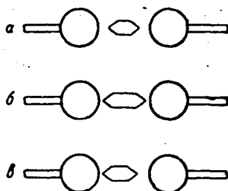
Fig. 7. Diagram of the arrangement of electrodes in experiments with the influence of the distance between pointed conical copper electrodes on the magnitude of erosion: a - steel balls at a great distance from the electrodes; b - steel balls at a short distance from the electrodes; c - one steel ball at a short distance from an electrode, and another ball at a long distance.
