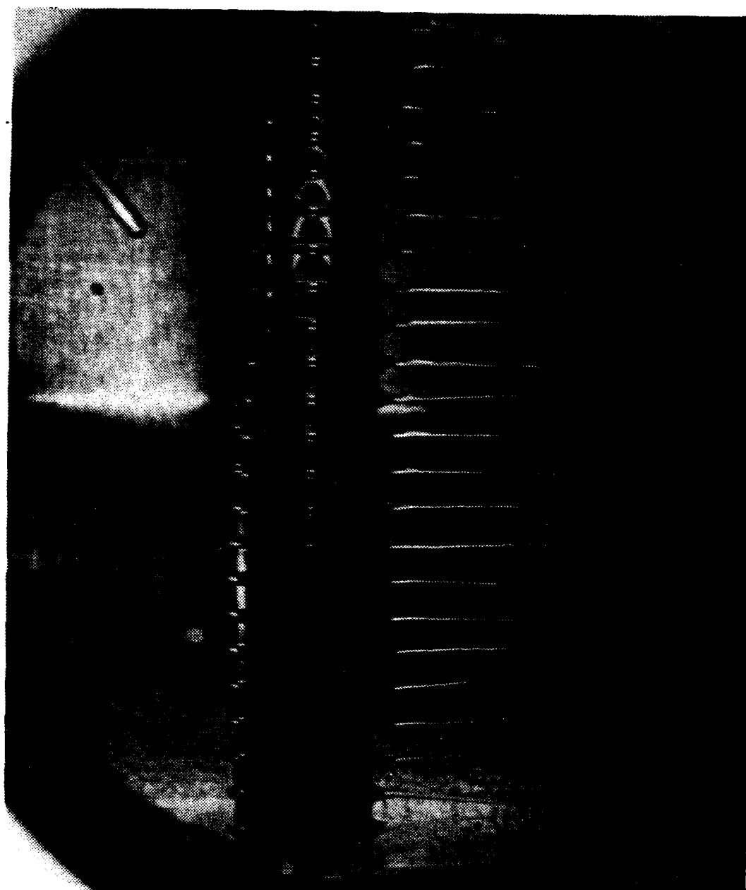
Figure 5.23 Photograph of Tube F08 Under High Heat Flux.
