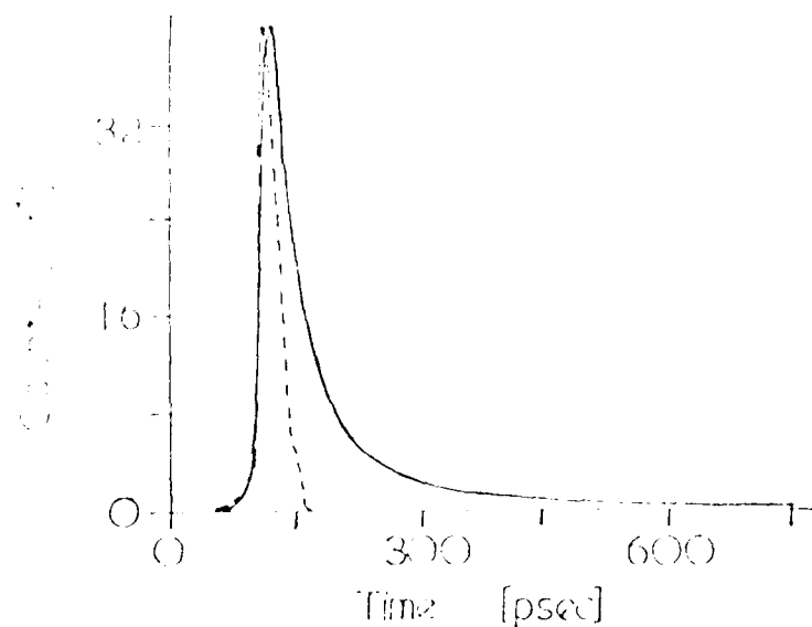
Figure 1. The nonexer decay of 2,5-dimethyl-2-thiophenol (solid curve), and nonexer decay of 2,5-dimethyl-2-thiophenol (dashed curve) [16].
