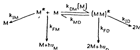
Scheme 1 Kinetic scheme for excimer formation and decay after Birks
