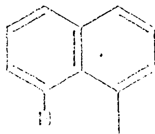
PERYLENE IN DAPHESED ETFA ( ^{10}\text{P}/^{10}\text{CH}_2 )
