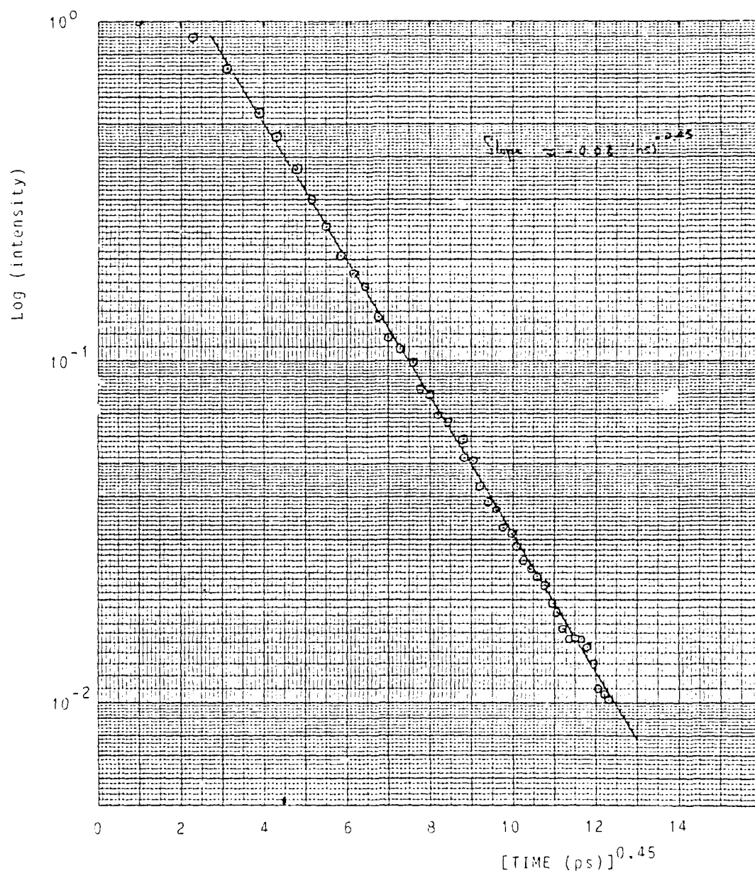
Figure 15 Fluorescence decay of PDA 10H, 4°K, plotted as log intensity vs. t_{0.45} .
