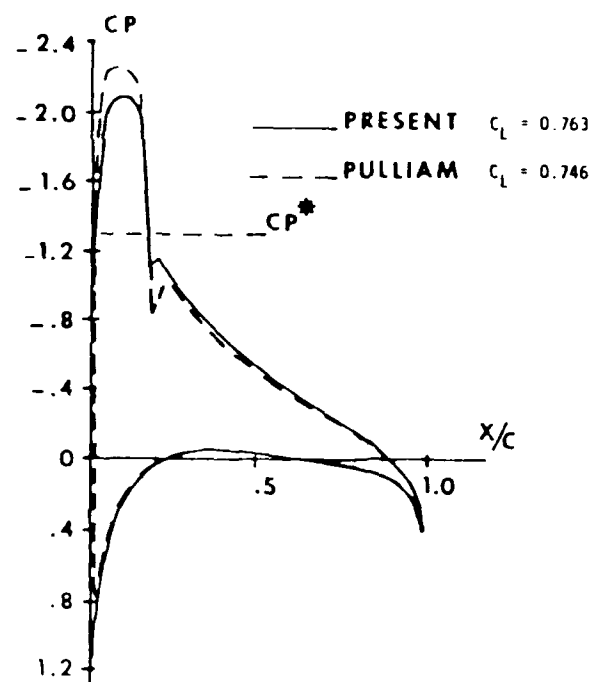
Figure B7(b). Pressure coefficients ( M_\infty = 0.60 , \beta_\infty = 5.0^\circ )
