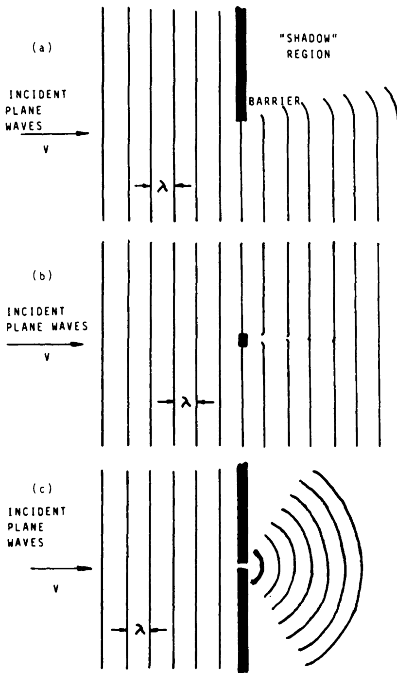
Figure 2.5 Diffraction of waves (a) around an object large compared to wavelength (b) around an object small compared to wavelength (c) through a small opening
