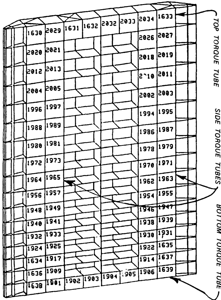
Figure 26. Torque-tube model 2
