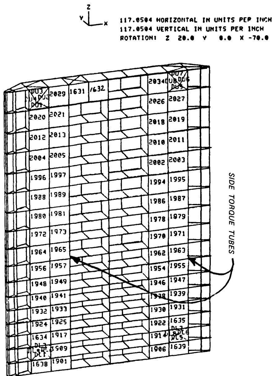
Figure 27. Torque-tube model 3
