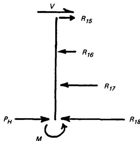
Figure 12. Static equilibrium at lower gusset plate
