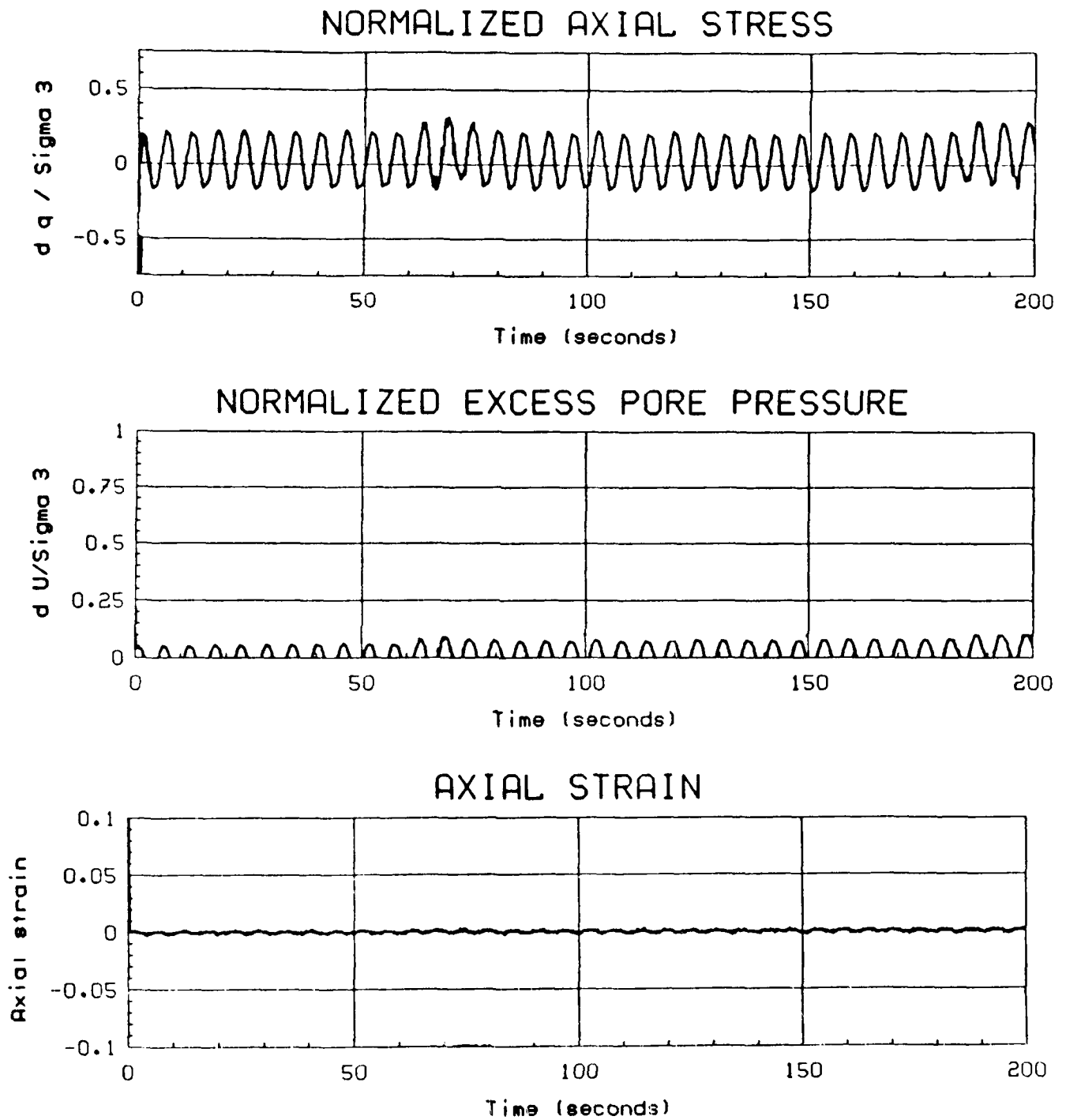
Figure 4-17: ISOTROPICALLY CONSOLIDATED UNDRAINED CYCLIC TRIAXIAL TEST NO. 38
