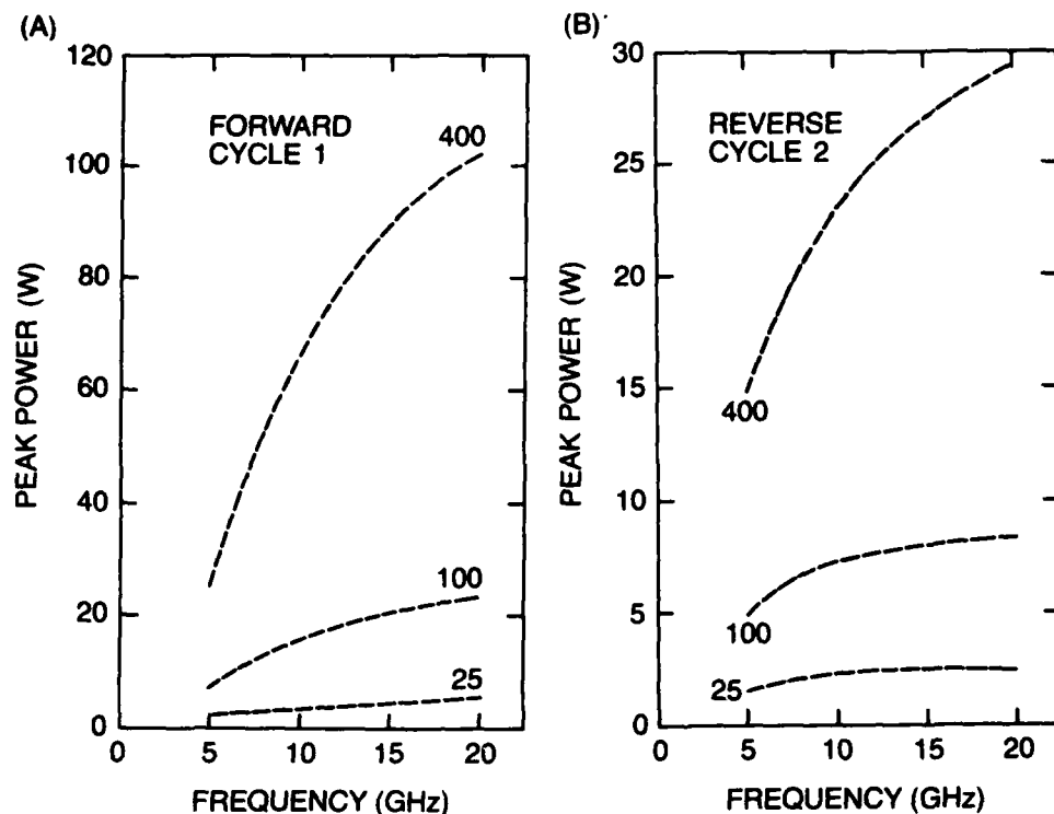
Figure 13. Power dissipated in 1-μm diode as a function of frequency for three average input powers in watts: (a) initial forward half-cycle and (b) following reverse half-cycle.
